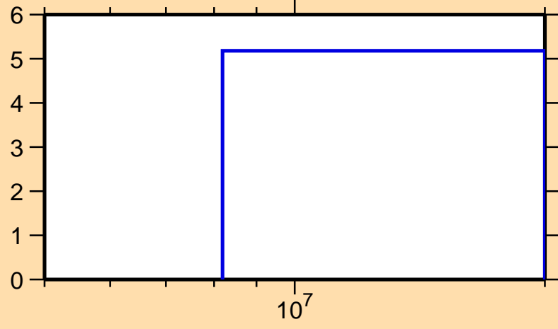
\Delta\sigma/\sigma vs. E for ^{230}\text{Rn}(n,el.)
