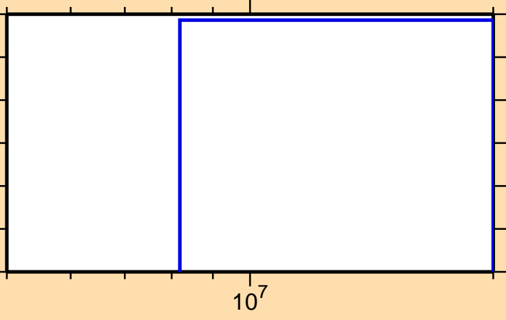
\sigma vs. E for ^{230}\text{Rn}(n,\alpha)
