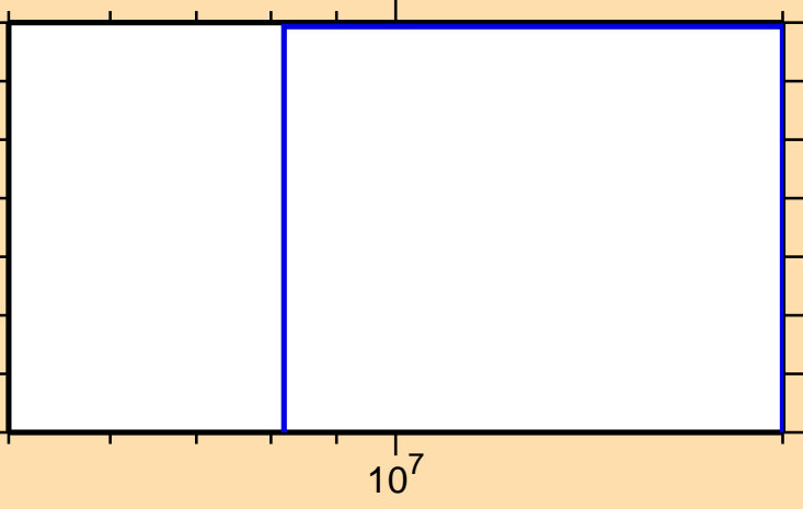
\sigma vs. E for ^{230}\text{Rn}(n,t)
