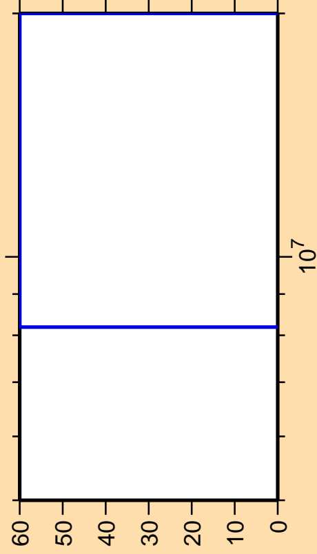
\Delta\sigma/\sigma vs. E for ^{230}\text{Rn}(n,nd)
