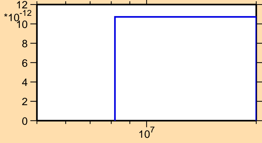
\sigma vs. E for ^{230}\text{Rn}(n,nd)
