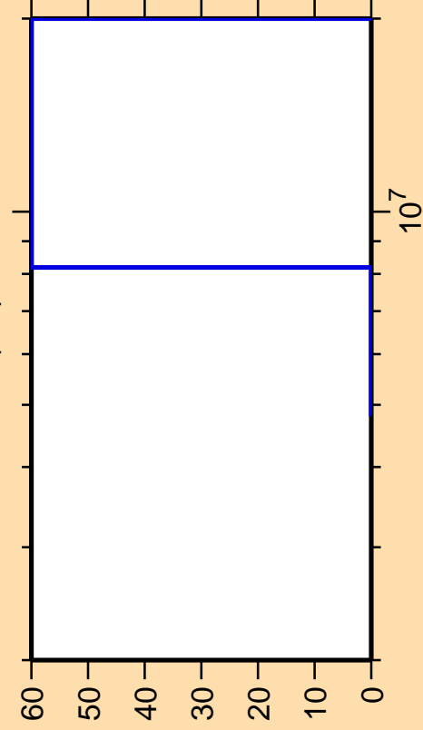
\Delta\sigma/\sigma vs. E for ^{230}\text{Rn}(n,f)
