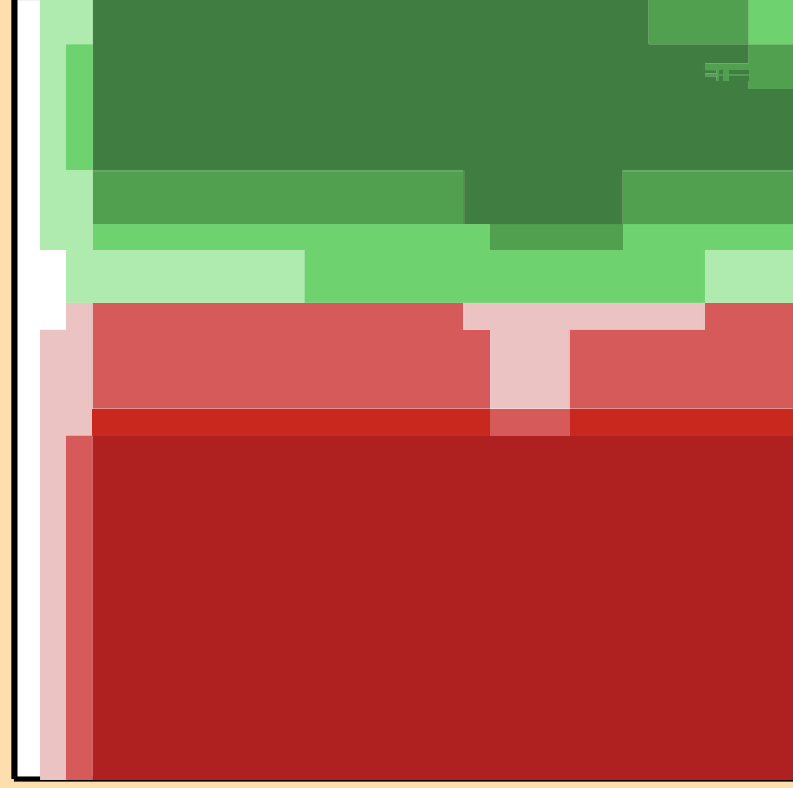
\Delta\sigma/\sigma vs. E for ^{88}\text{Ru}(n,n_1)
