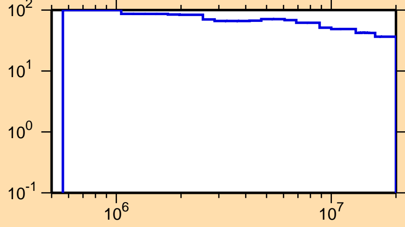
\Delta\sigma/\sigma vs. E for ^{88}\text{Ru}(n,\text{inel.})
