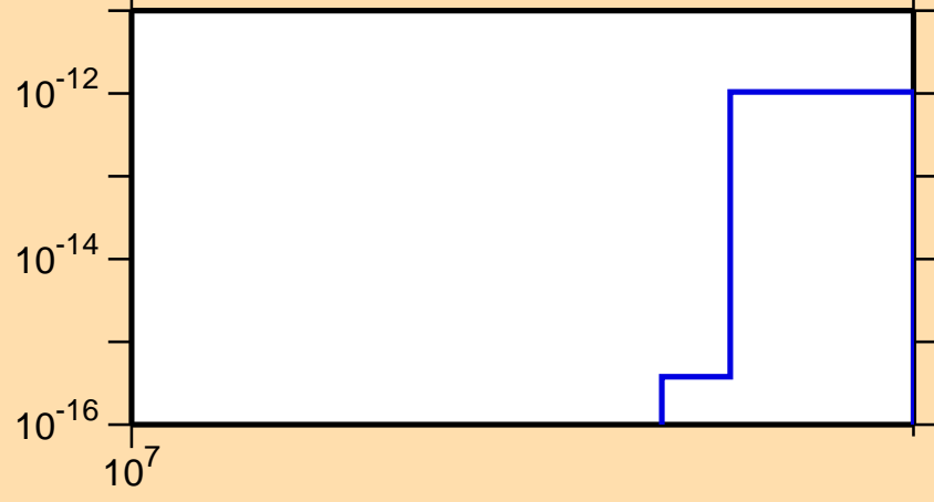
\sigma vs. E for ^{88}\text{Ru}(n,\text{nd})
