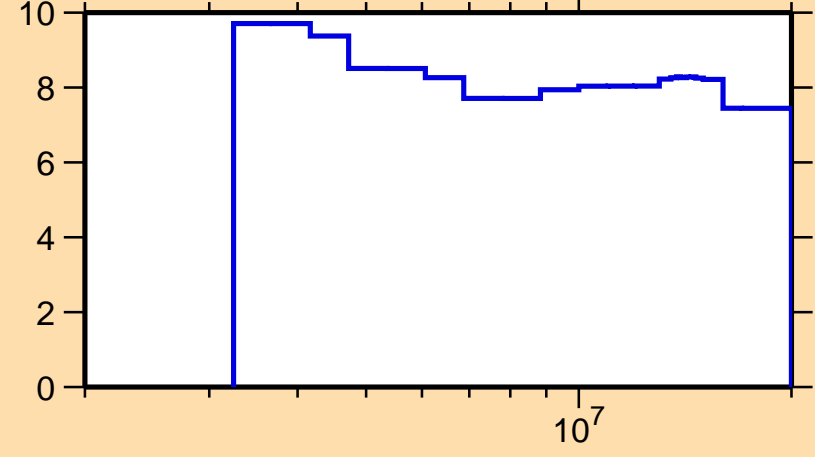
\Delta\sigma/\sigma vs. E for ^{88}\text{Ru}(n,n\text{onel.})
