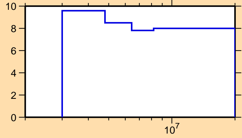
\Delta\sigma/\sigma vs. E for ^{88}\text{Ru}(n,n\text{inel.})
