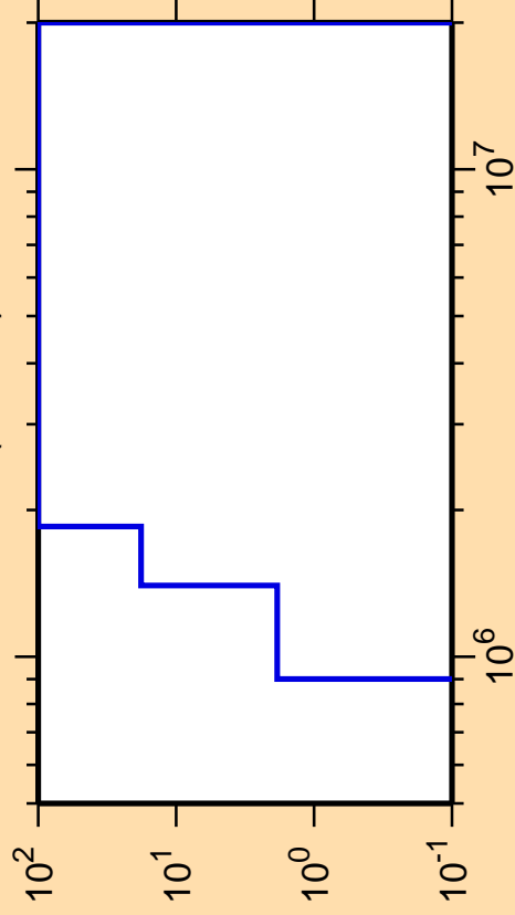
\Delta\sigma/\sigma vs. E for ^{88}\text{Ru}(n,\text{He}3)
