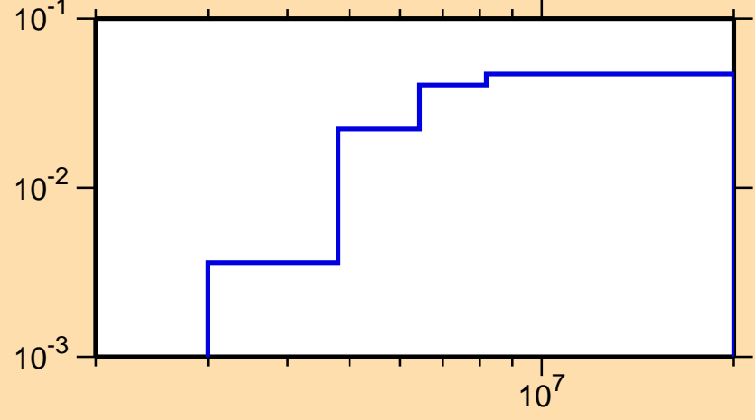
\sigma vs. E for ^{88}\text{Ru}(n,n\text{cont.})
