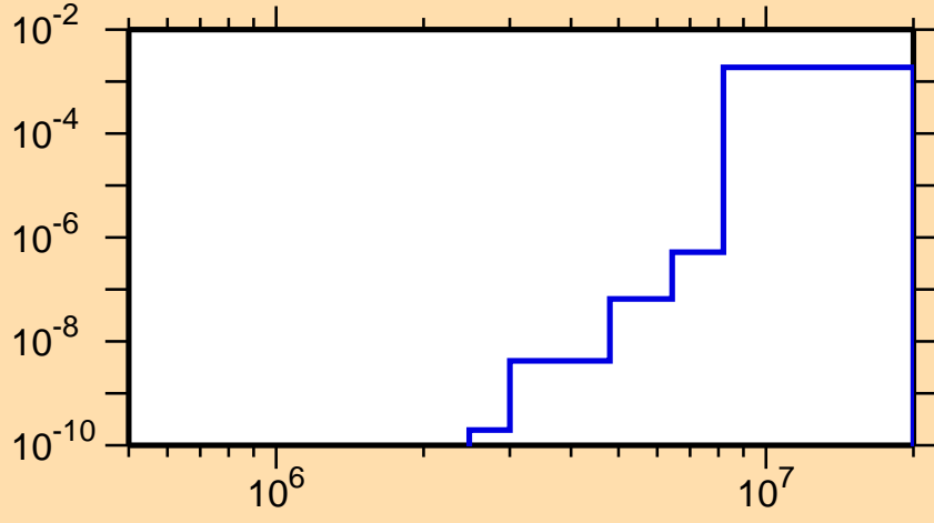
\sigma vs. E for ^{88}\text{Ru}(n,\text{He}3)
