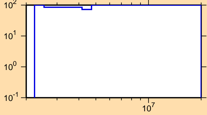
\Delta\sigma/\sigma vs. E for ^{89}\text{Ru}(n,n\text{cont.})
