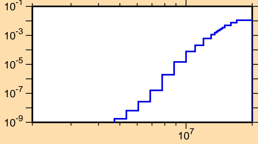
\sigma vs. E for ^{89}\text{Ru}(n,\text{He}3)
