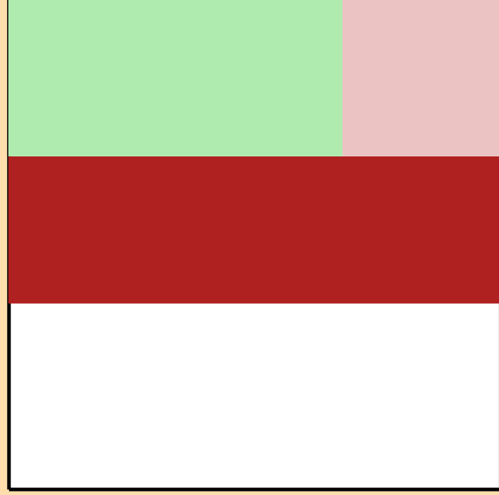
\Delta\sigma/\sigma vs. E for ^{89}\text{Ru}(n,\text{nonel.})
