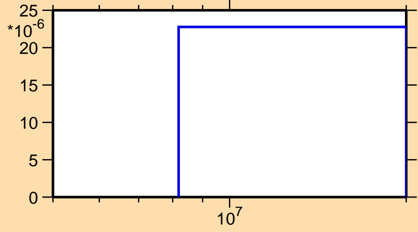
\sigma vs. E for ^{89}\text{Ru}(n,2n)
