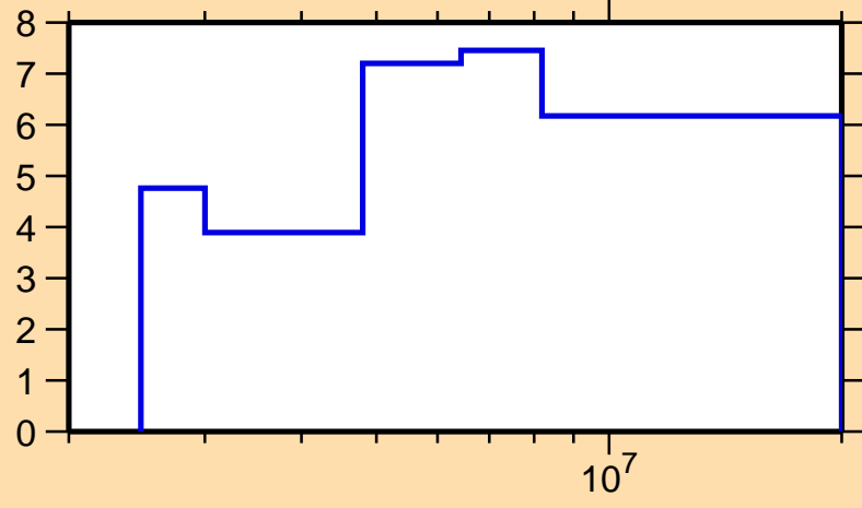
\Delta\sigma/\sigma vs. E for ^{89}\text{Ru}(n, el.)
