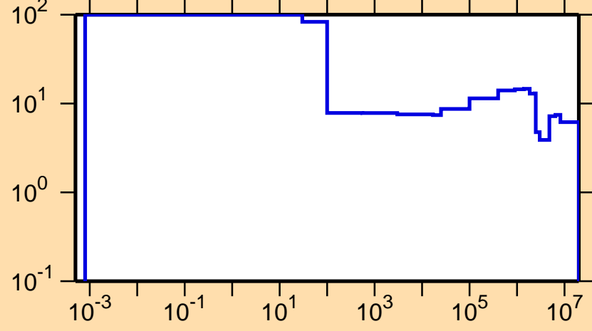
\Delta\sigma/\sigma vs. E for ^{89}\text{Ru}(n,\text{el.})
