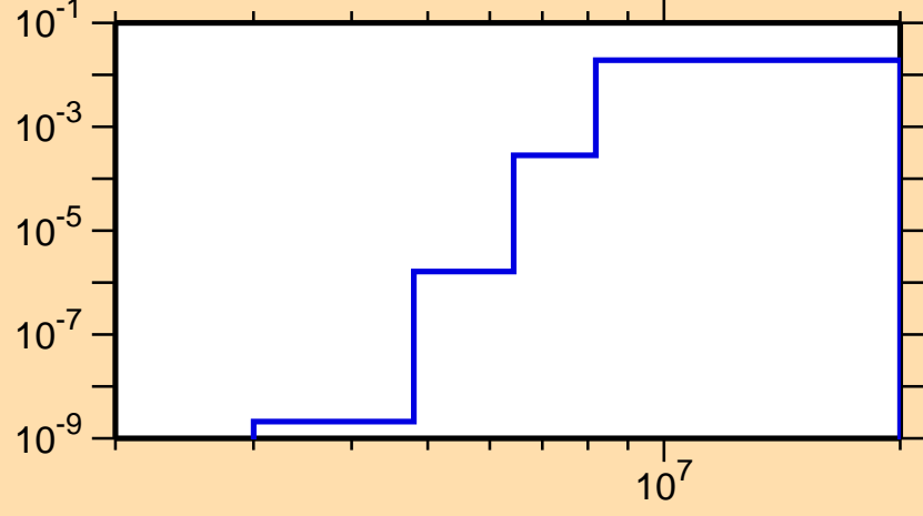
\sigma vs. E for ^{89}\text{Ru}(n,d)
