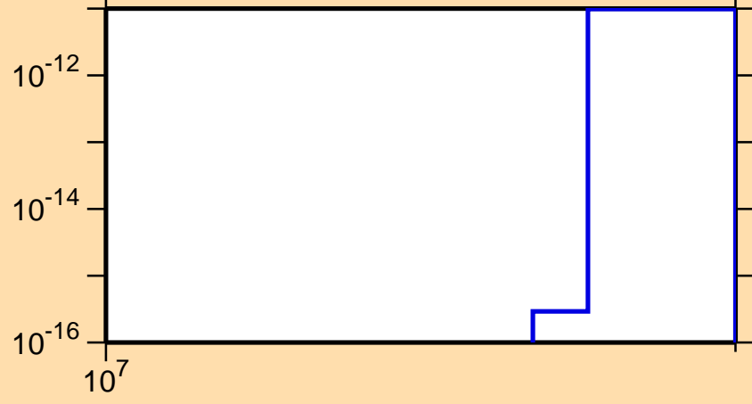
\sigma vs. E for ^{90}\text{Ru} (mt 34)
