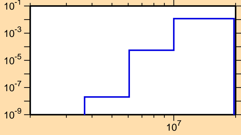
\sigma vs. E for ^{90}\text{Ru}(n,d)
