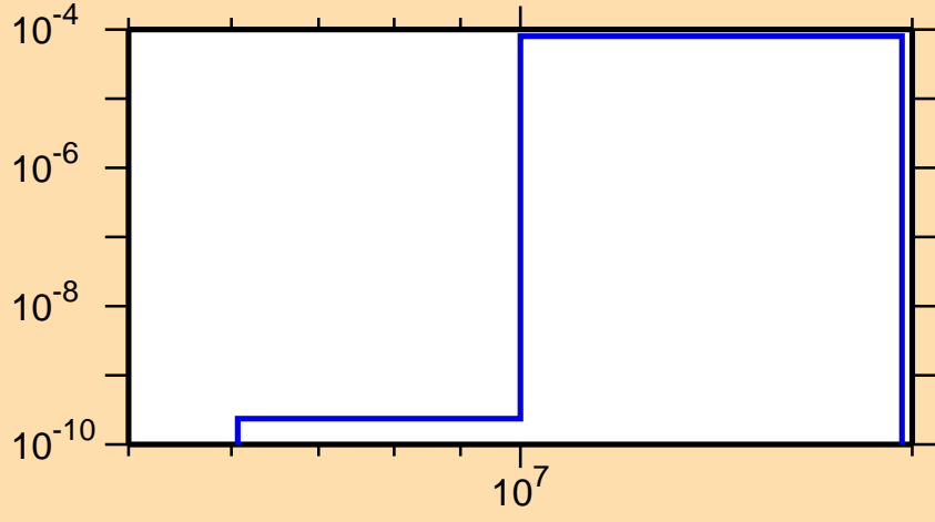
\sigma vs. E for ^{90}\text{Ru}(n,\alpha)
