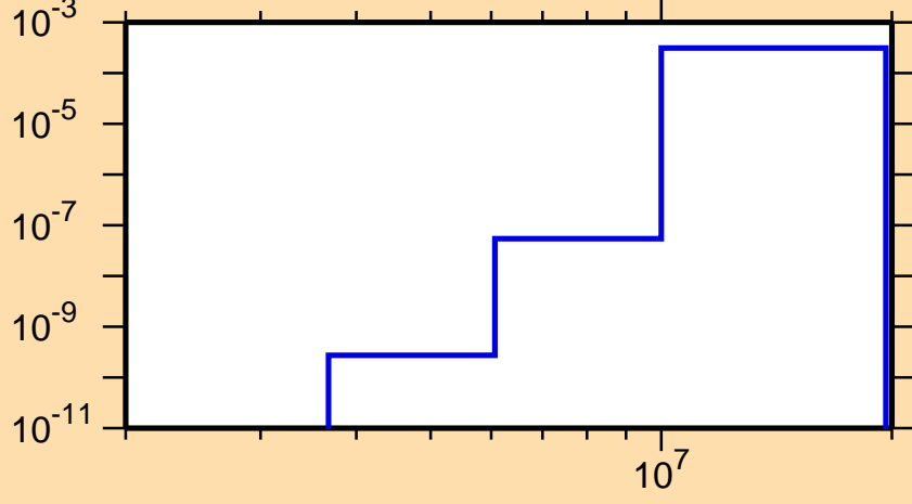
\sigma vs. E for ^{90}\text{Ru}(n,\text{He}3)
