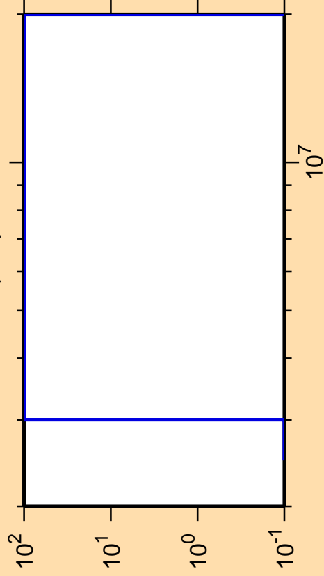
\Delta\sigma/\sigma vs. E for ^{90}\text{Ru}(n,d)
