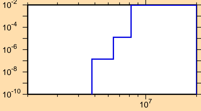
\sigma vs. E for ^{90}\text{Ru}(n,d)
