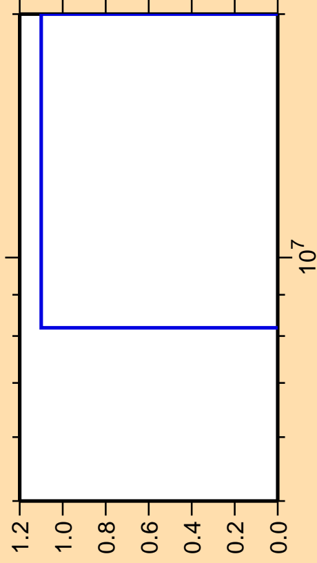
\Delta\sigma/\sigma vs. E for ^{90}\text{Ru}(n,nd)
