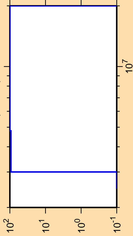
\Delta\sigma/\sigma vs. E for ^{90}\text{Ru}(n,\text{He}3)
