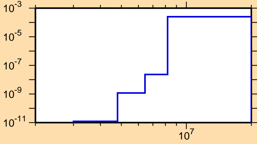
\sigma vs. E for ^{90}\text{Ru}(n,\text{He}3)
