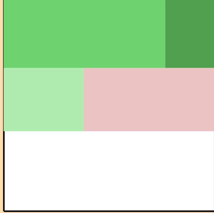
\Delta\sigma/\sigma vs. E for ^{91}\text{Ru}(n,\text{nonel.})
