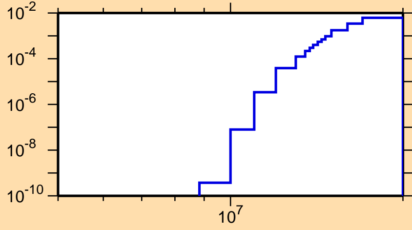
\sigma vs. E for ^{91}\text{Ru}(n,pd)
