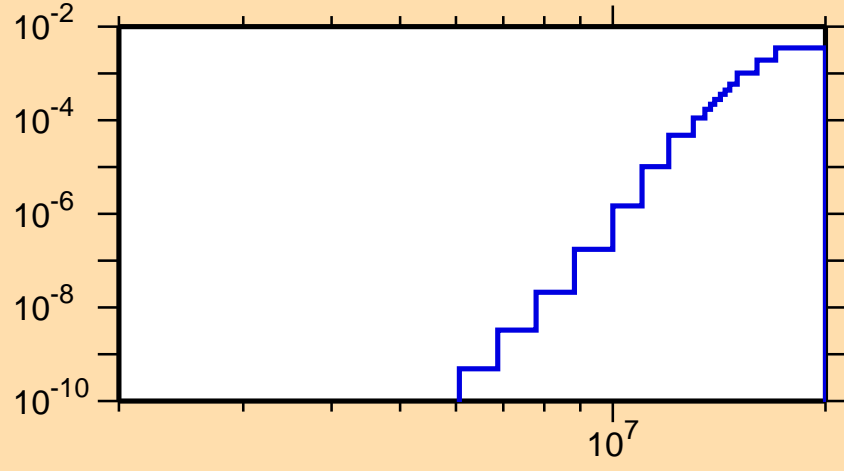
\sigma vs. E for ^{91}\text{Ru}(n,\text{He}3)
