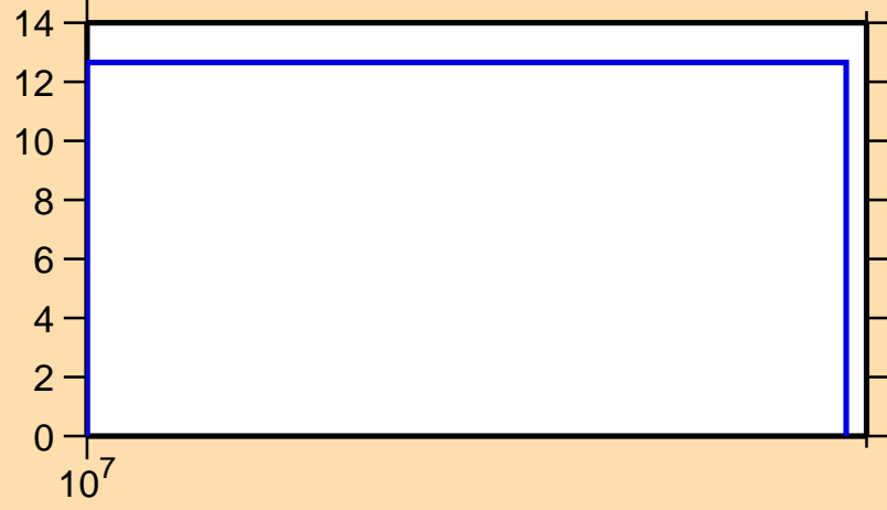
\Delta\sigma/\sigma vs. E for ^{91}\text{Ru}(n,\text{el.})
