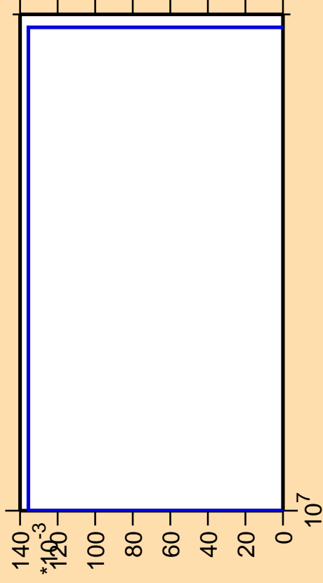
\Delta\sigma/\sigma vs. E for ^{91}\text{Ru}(\text{mt117})
