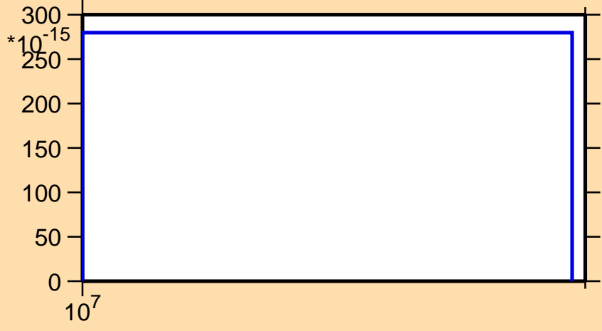
\sigma vs. E for ^{91}\text{Ru}(\text{mt117})
