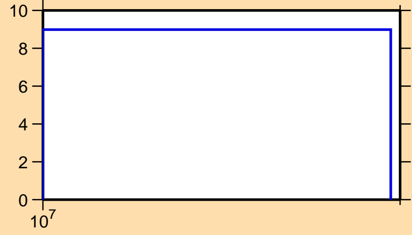
\Delta\sigma/\sigma vs. E for ^{91}\text{Ru}(n,\text{tot.})
