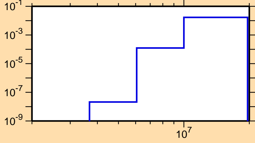
\sigma vs. E for ^{91}\text{Ru}(n,d)
