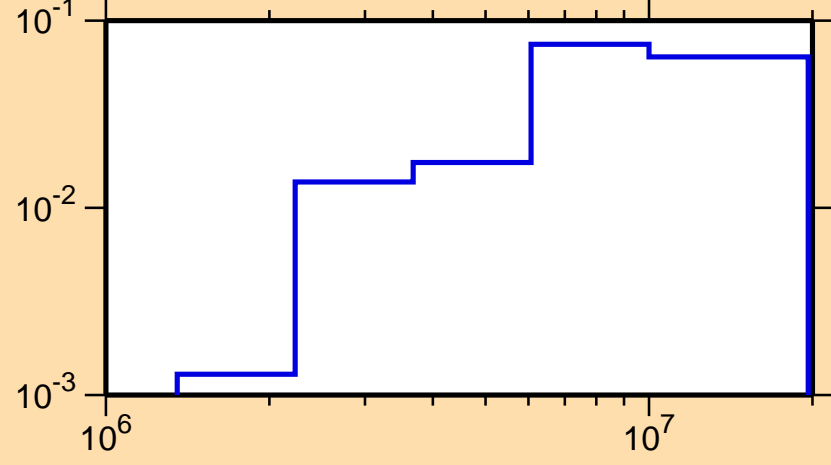
\sigma vs. E for ^{91}\text{Ru}(n,n\text{cont.})
