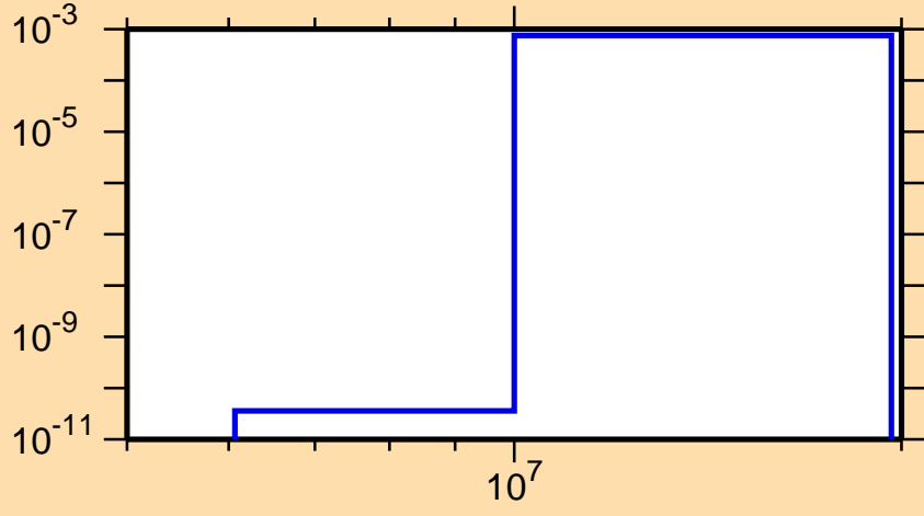
\sigma vs. E for ^{91}\text{Ru}(n,\text{pd})
