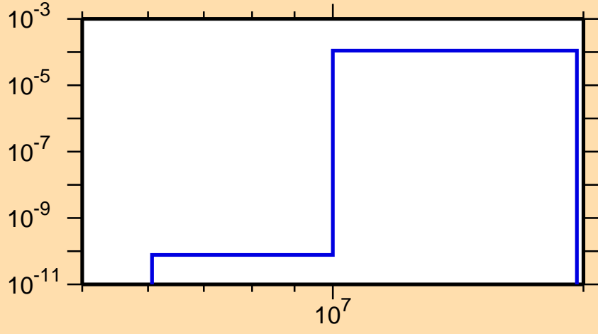
\sigma vs. E for ^{91}\text{Ru}(n,n\alpha)
