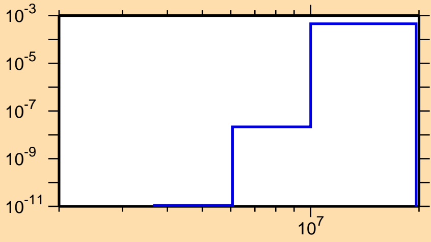
\sigma vs. E for ^{91}\text{Ru}(n,\text{He}3)
