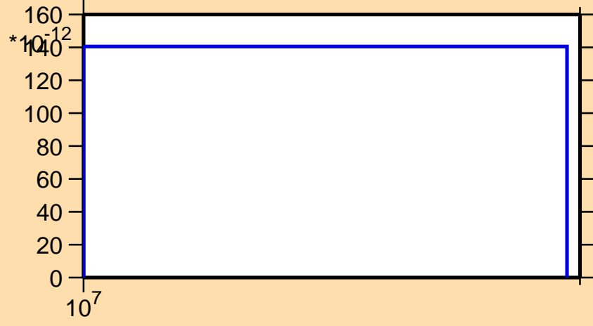
\sigma vs. E for ^{91}\text{Ru} (mt 34)
