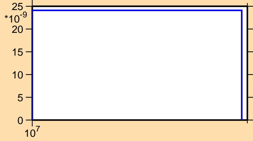
\sigma vs. E for ^{91}\text{Ru}(n,2np)
