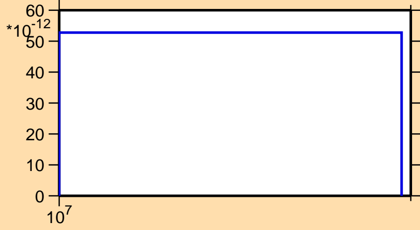
\sigma vs. E for ^{91}\text{Ru} (mt 45)
