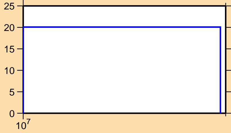
\Delta\sigma/\sigma vs. E for ^{91}\text{Ru}(n,\text{inel.})
