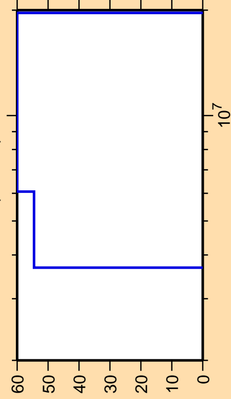
\Delta\sigma/\sigma vs. E for ^{91}\text{Ru}(n,\text{He}3)
