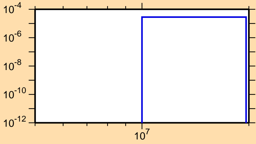
\sigma vs. E for ^{91}\text{Ru}(n,t)
