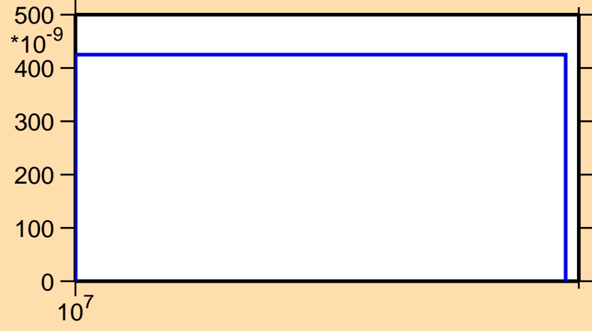
\sigma vs. E for ^{91}\text{Ru}(n,pt)
