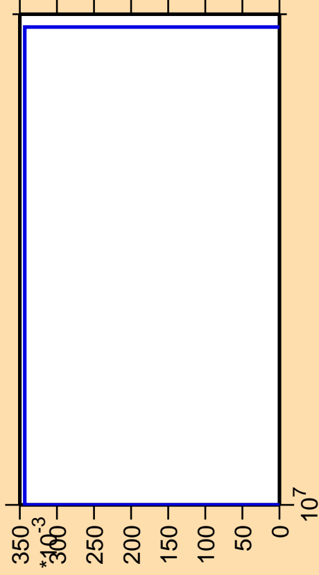
\Delta\sigma/\sigma vs. E for ^{93}\text{Ru} (mt 45)
