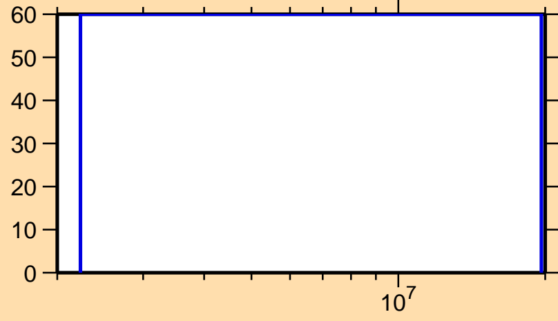
\Delta\sigma/\sigma vs. E for ^{93}\text{Ru}(n,n\text{cont.})
