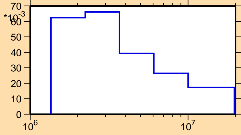
\sigma vs. E for ^{93}\text{Ru}(n,n_3)
