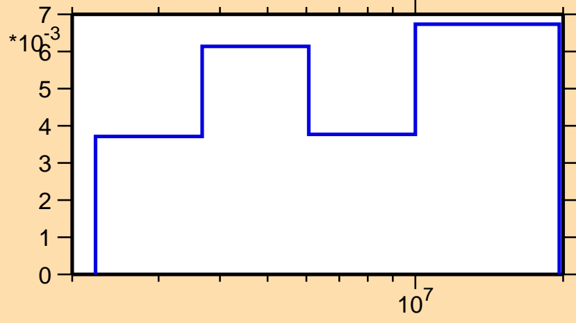
\sigma vs. E for ^{93}\text{Ru}(n,n\text{cont.})
