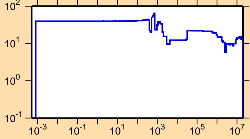
\Delta\sigma/\sigma vs. E for ^{94}\text{Ru}(n,\text{el.})
