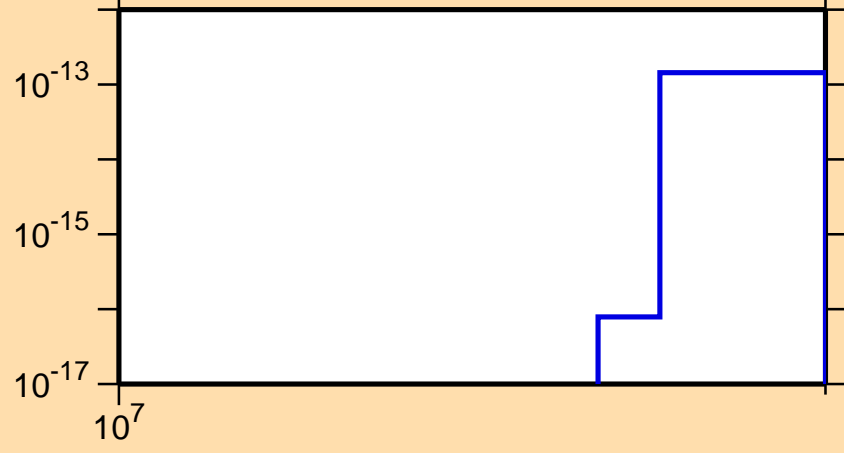
\sigma vs. E for ^{94}\text{Ru}(\text{mt117})
