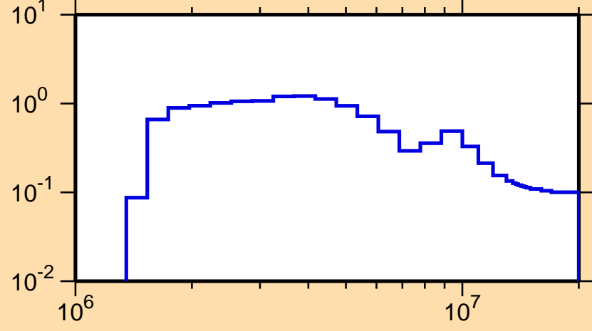
\sigma vs. E for ^{94}\text{Ru}(n,\text{inel.})
