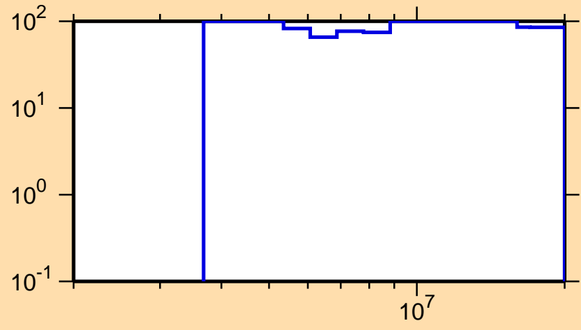
\Delta\sigma/\sigma vs. E for ^{94}\text{Ru}(n,ncont.)
