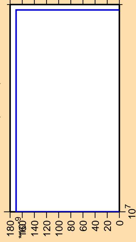
\Delta\sigma/\sigma vs. E for ^{94}\text{Ru}(n,2n\alpha)
