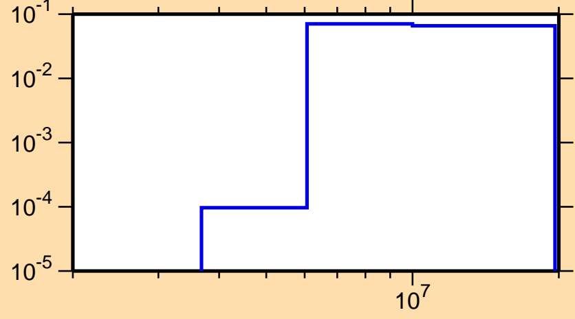
\sigma vs. E for ^{94}\text{Ru}(n,n\text{cont.})
