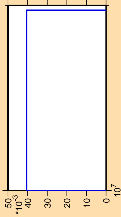
\Delta\sigma/\sigma vs. E for ^{94}\text{Ru}(\text{mt } 45)
