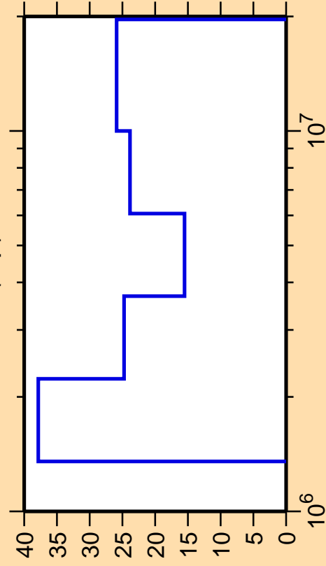
\Delta\sigma/\sigma vs. E for ^{94}\text{Ru}(n,p)
