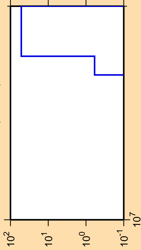
\Delta\sigma/\sigma vs. E for ^{95}\text{Ru}(\text{mt117})
