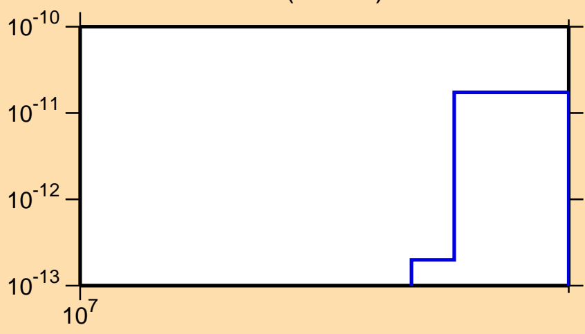
\sigma vs. E for ^{95}\text{Ru}(\text{mt117})
