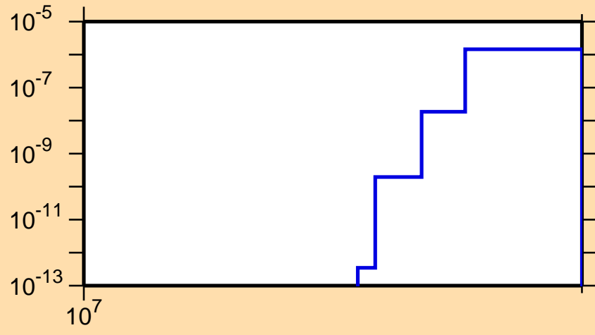
\sigma vs. E for ^{95}\text{Ru}(n,\text{pt})
