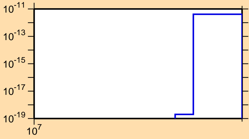
\sigma vs. E for ^{95}\text{Ru}(n,2n\alpha)
