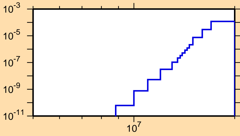
\sigma vs. E for ^{95}\text{Ru}(n,\text{He}3)
