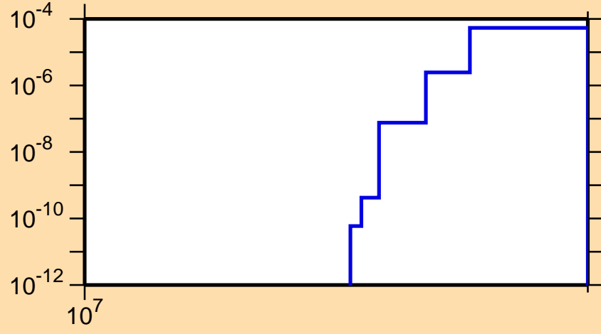
\sigma vs. E for ^{95}\text{Ru}(n,\text{nd})
