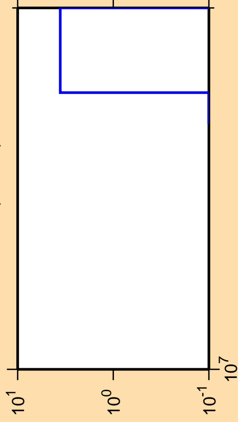
\Delta\sigma/\sigma vs. E for ^{95}\text{Ru}(n,2n\alpha)
