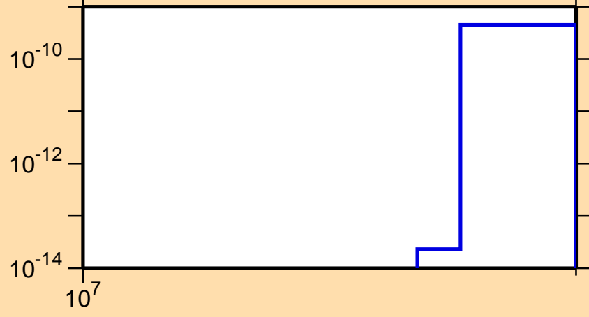
\sigma vs. E for ^{95}\text{Ru} (mt 45)
