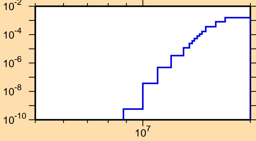
\sigma vs. E for ^{95}\text{Ru}(n,t)
