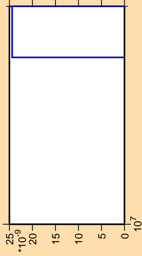
\Delta\sigma/\sigma vs. E for ^{95}\text{Ru}(n,nt)
