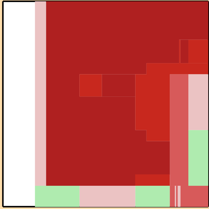
\Delta\sigma/\sigma vs. E for ^{95}\text{Ru}(n,n\text{cont.})
