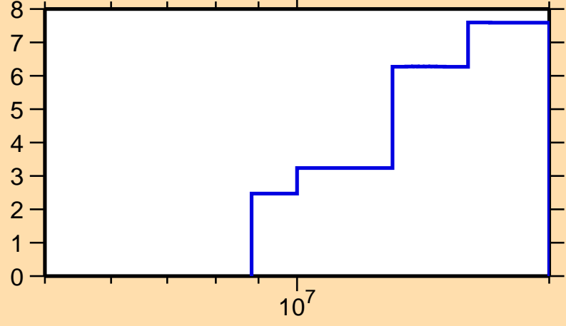
\Delta\sigma/\sigma vs. E for ^{95}\text{Ru}(n,\text{tot.})
