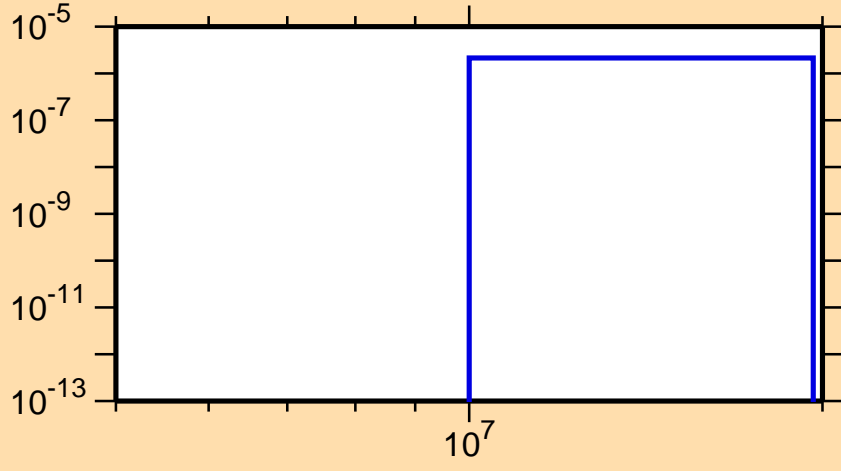
\sigma vs. E for ^{95}\text{Ru}(n,pd)
