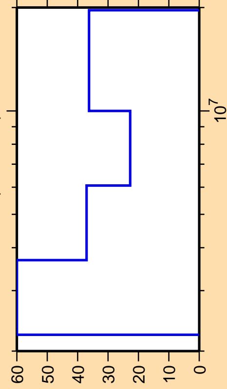
\Delta\sigma/\sigma vs. E for ^{95}\text{Ru}(n,\text{ncont.})
