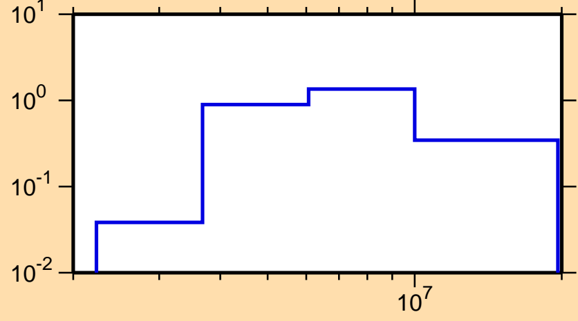
\sigma vs. E for ^{95}\text{Ru}(n,n\text{cont.})
