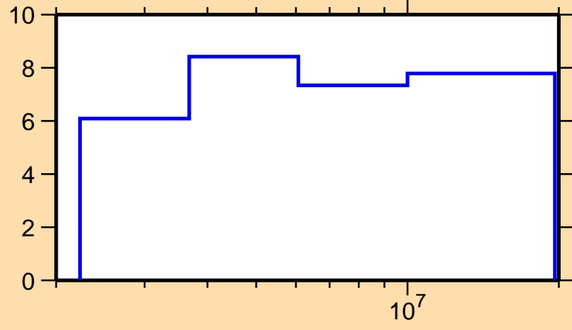
\Delta\sigma/\sigma vs. E for ^{95}\text{Ru}(n,n\text{onel.})
