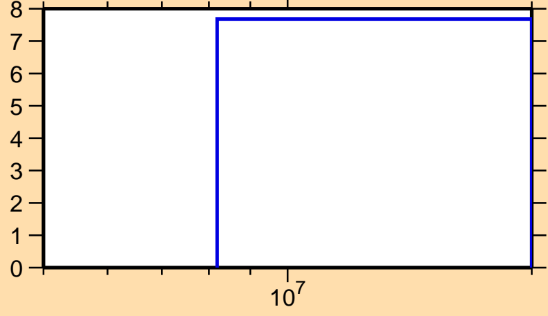
\Delta\sigma/\sigma vs. E for ^{95}\text{Ru}(n,\text{nonel.})
