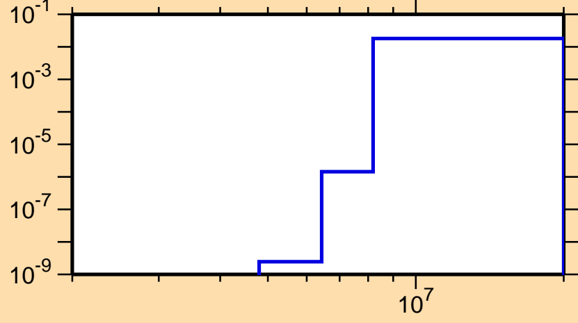
\sigma vs. E for ^{95}\text{Ru}(n,p\alpha)
