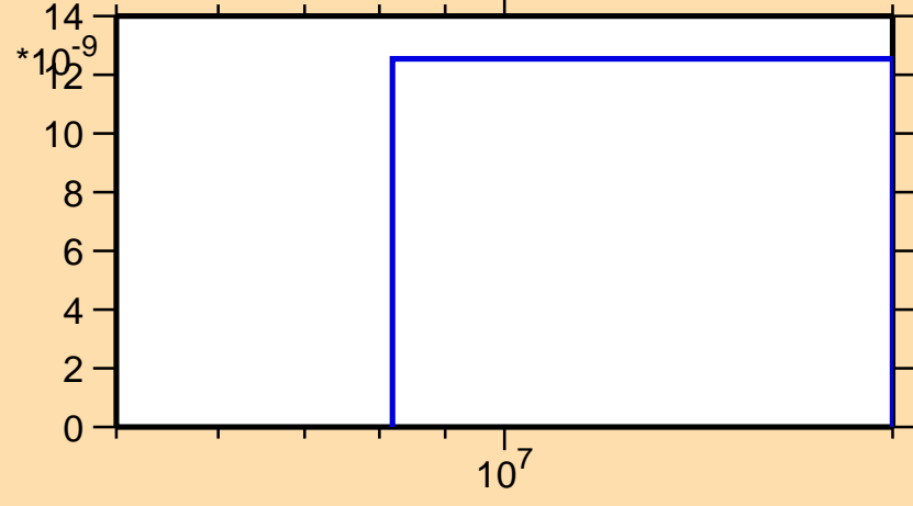
\sigma vs. E for ^{95}\text{Ru}(n,\text{pt})
