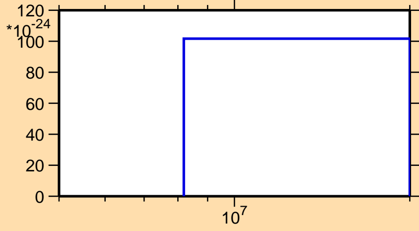
\sigma vs. E for ^{95}\text{Ru}(n,nt)
