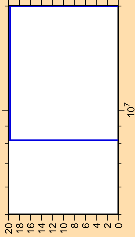
\Delta\sigma/\sigma vs. E for ^{95}\text{Ru}(\text{mt } 34)
