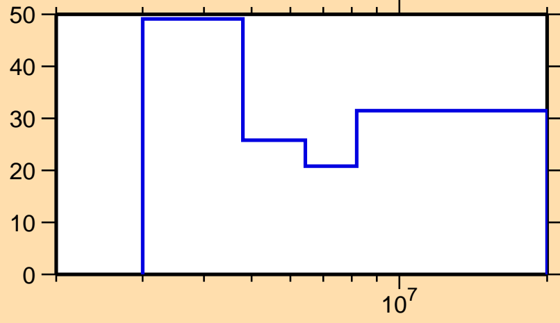
\Delta\sigma/\sigma vs. E for ^{95}\text{Ru}(n,n\text{cont.})
