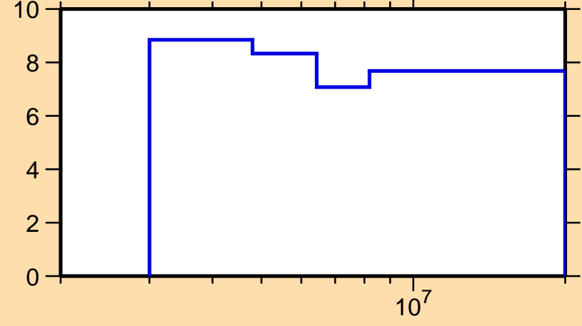
\Delta\sigma/\sigma vs. E for ^{95}\text{Ru}(n,n\text{onrel.})
