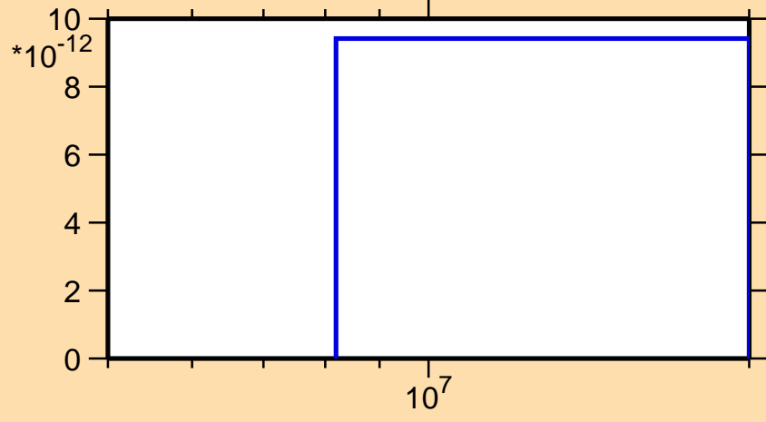
\sigma vs. E for ^{95}\text{Ru}(\text{mt } 34)
