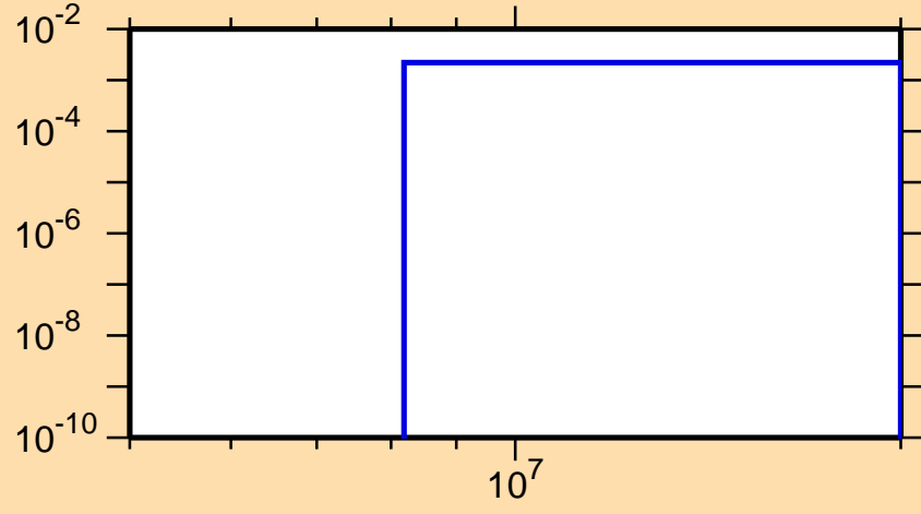
\sigma vs. E for ^{95}\text{Ru}(n,\alpha)
