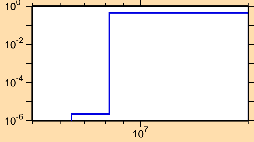
\sigma vs. E for ^{95}\text{Ru}(n,np)
