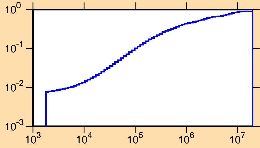
\mu vs. E for ^{98}\text{Ru}(\text{mt251})
