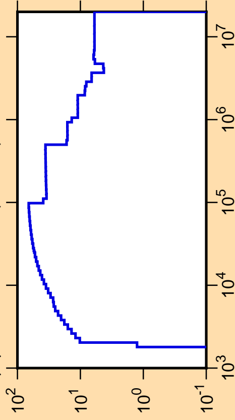
\Delta\mu/\mu vs. E for ^{98}\text{Ru}(\text{mt251})
