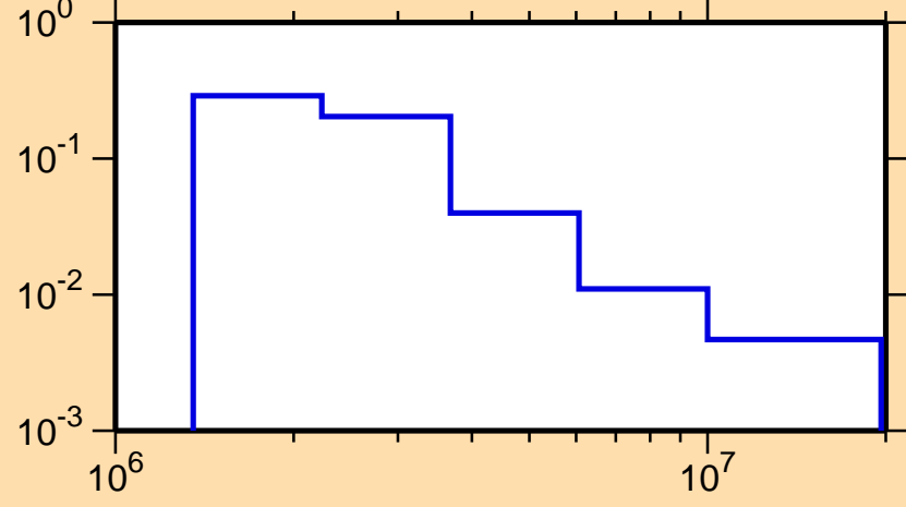
\sigma vs. E for ^{98}\text{Ru}(n,n_4)
