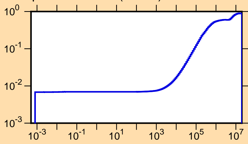
\mu vs. E for ^{99}\text{Ru}(\text{mt251})
