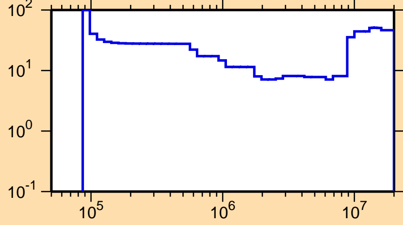
\Delta\sigma/\sigma vs. E for ^{99}\text{Ru}(n,\text{inel.})
