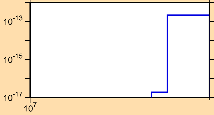
\sigma vs. E for ^{99}\text{Ru} (mt 45)
