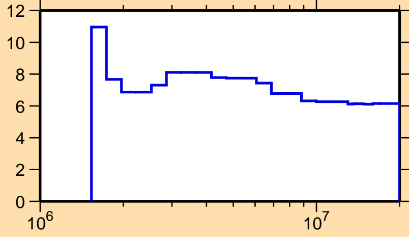
\Delta\sigma/\sigma vs. E for ^{99}\text{Ru}(n,n\text{onel.})
