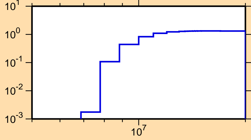
\sigma vs. E for ^{99}\text{Ru}(n,2n)
