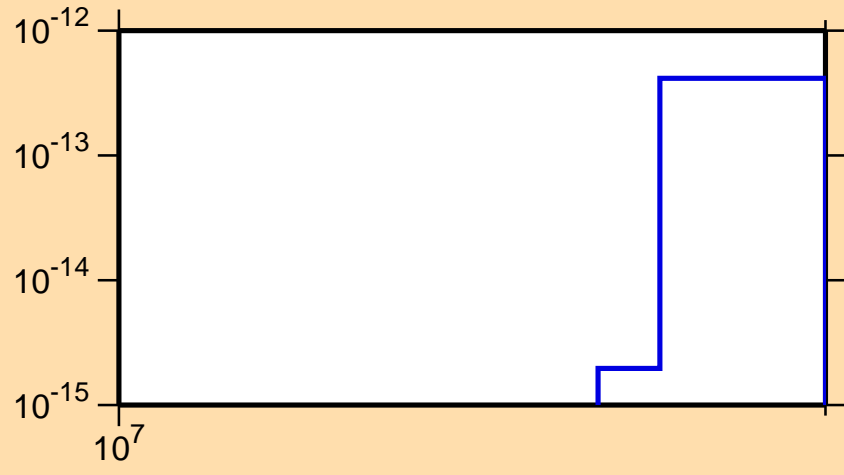
\sigma vs. E for ^{99}\text{Ru} (mt 34)
