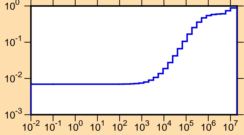
\mu vs. E for ^{99}\text{Ru}(\text{mt251})
