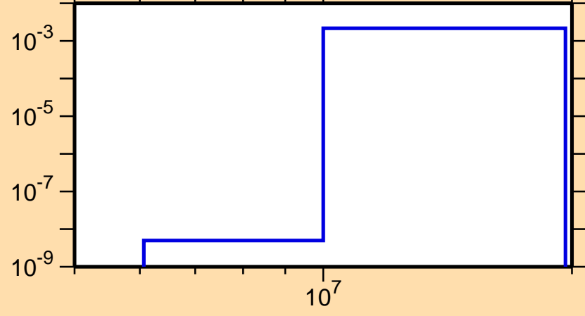
\sigma vs. E for ^{99}\text{Ru}(n,d)
