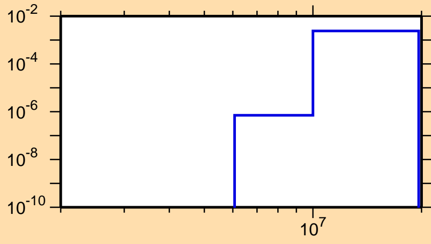
\sigma vs. E for ^{99}\text{Ru}(n,\alpha)
