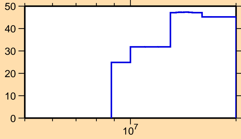
\Delta\sigma/\sigma vs. E for ^{100}\text{Ru}(n,\text{inel.})
