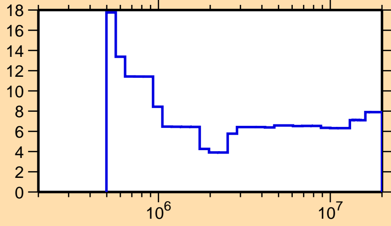
\Delta\sigma/\sigma vs. E for ^{100}\text{Ru}(n,\text{nonel.})
