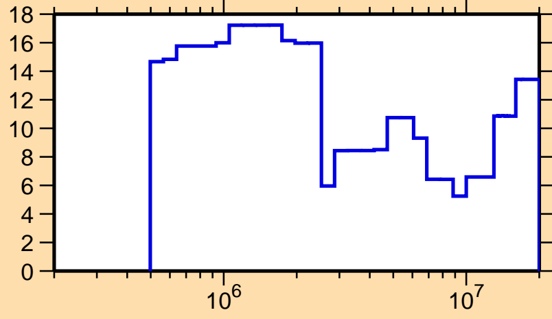
\Delta\sigma/\sigma vs. E for ^{100}\text{Ru}(n,\text{el.})
