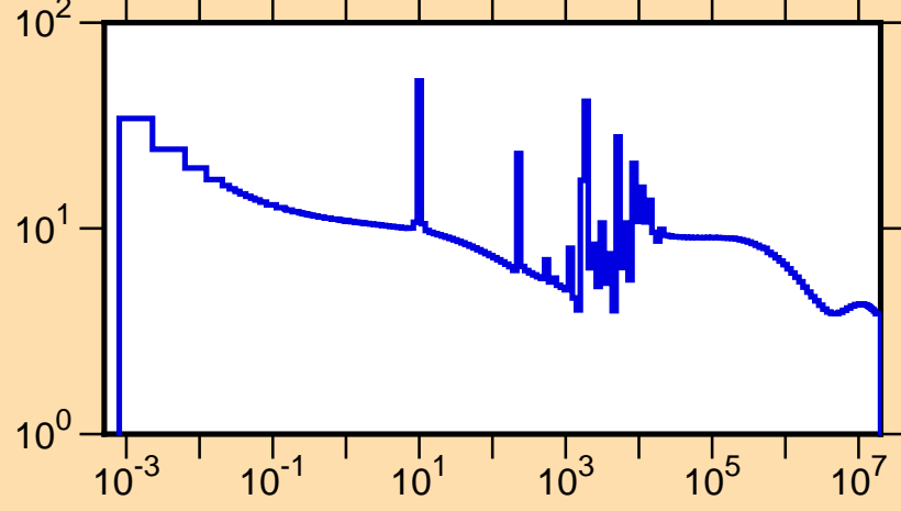
\sigma vs. E for ^{100}\text{Ru}(n,\text{tot.})
