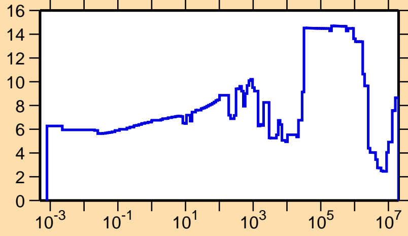
\Delta\sigma/\sigma vs. E for ^{100}\text{Ru}(n,\text{tot.})
