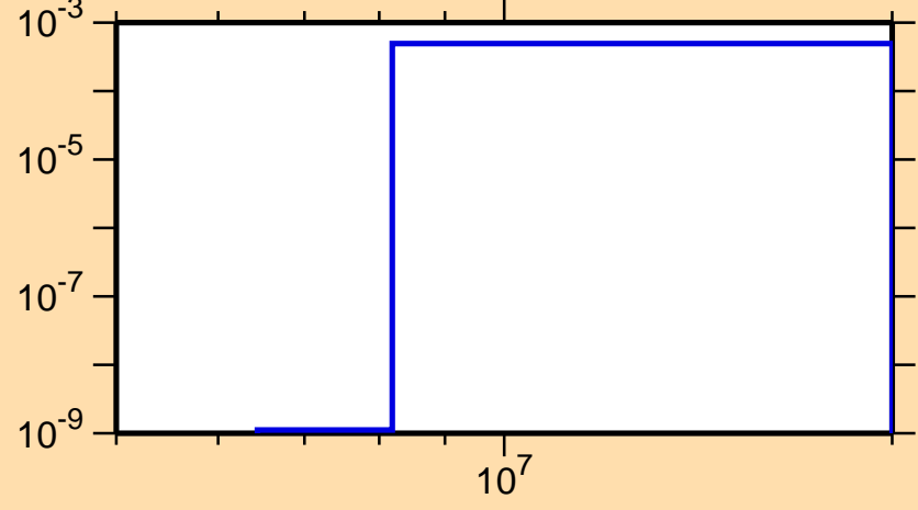
\sigma vs. E for ^{100}\text{Ru}(n,n\alpha)
