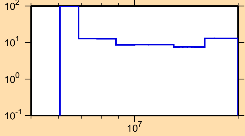
\Delta\sigma/\sigma vs. E for ^{101}\text{Ru}(n,2n)
