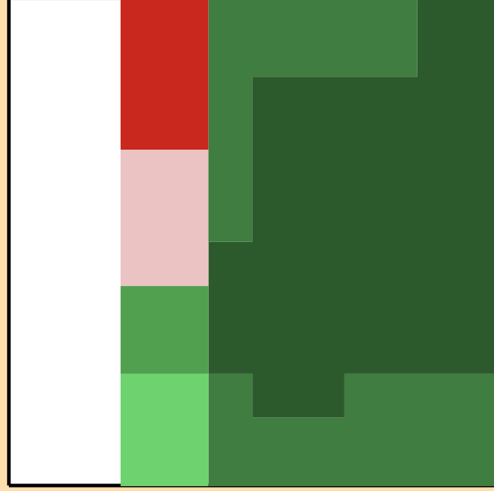
\Delta\sigma/\sigma vs. E for ^{101}\text{Ru}(n,2n)
