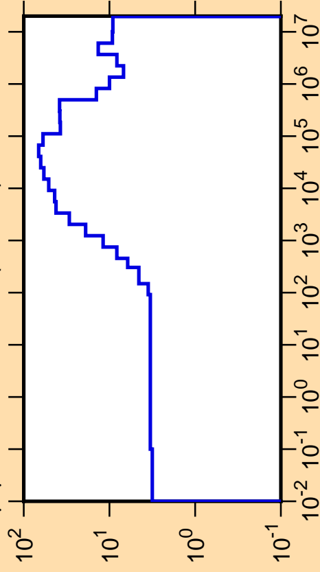
\Delta\mu/\mu vs. E for ^{101}\text{Ru}(\text{mt251})
