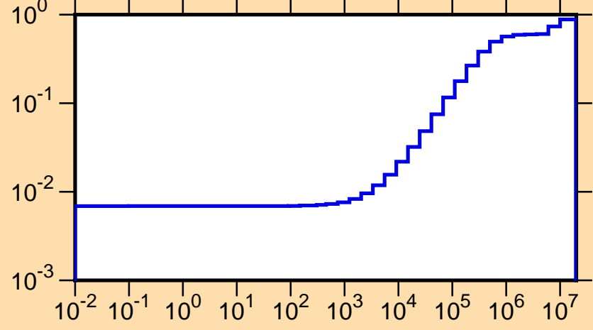
\mu vs. E for ^{101}\text{Ru}(\text{mt251})
