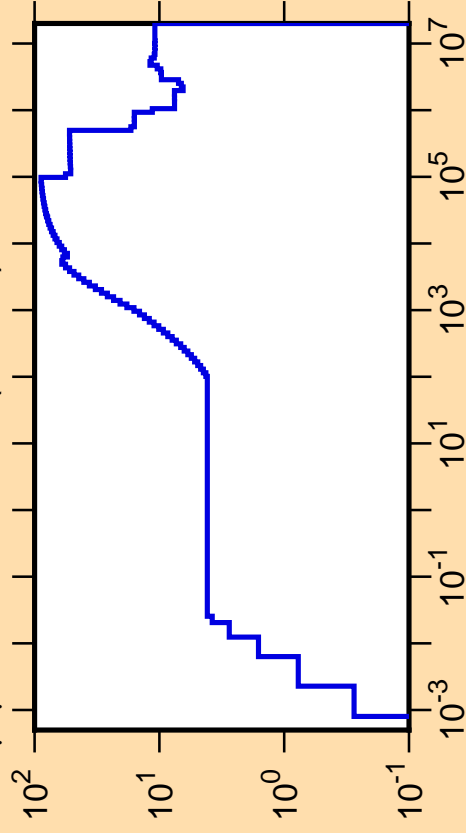
\Delta\mu/\mu vs. E for ^{103}\text{Ru}(\text{mt251})
