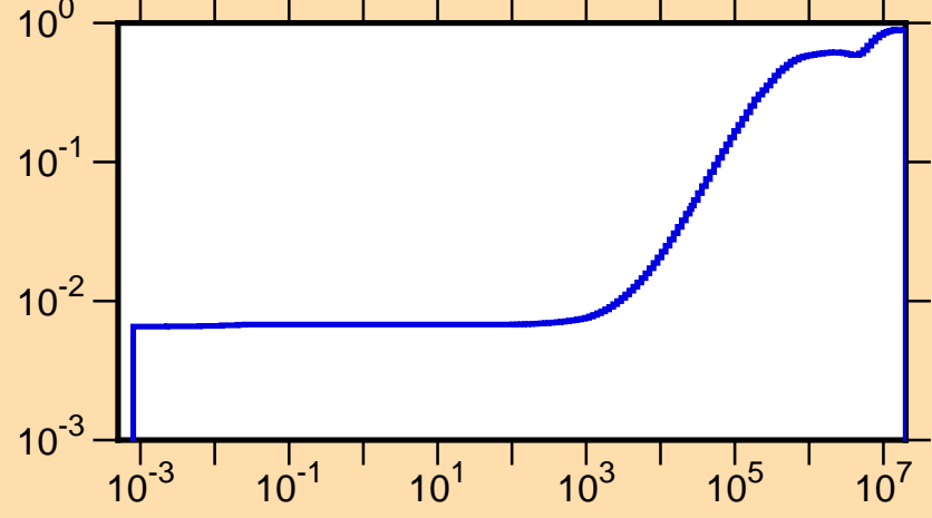
\mu vs. E for ^{103}\text{Ru}(\text{mt251})
