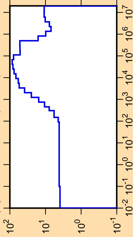
\Delta\mu/\mu vs. E for ^{103}\text{Ru}(\text{mt251})
