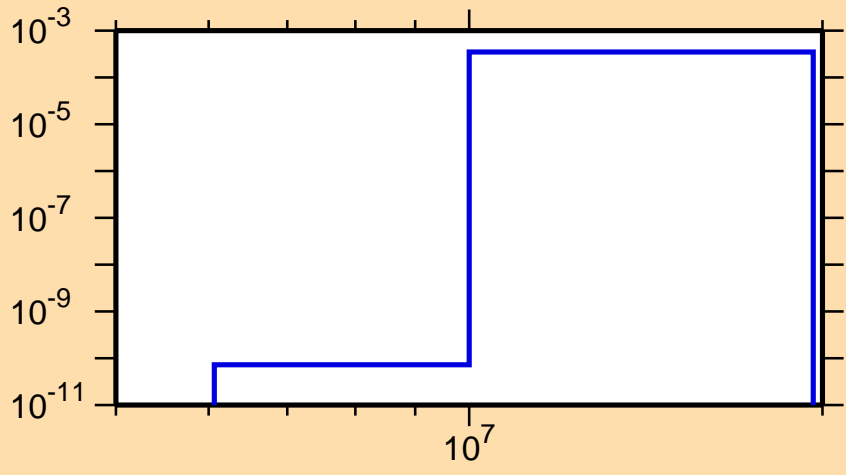
\sigma vs. E for ^{103}\text{Ru}(n,n\alpha)
