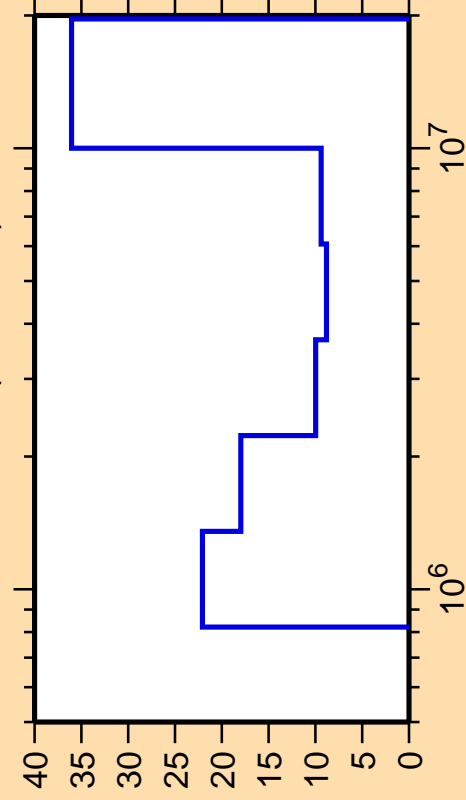
\Delta\sigma/\sigma vs. E for ^{103}\text{Ru}(n,\text{ncont.})
