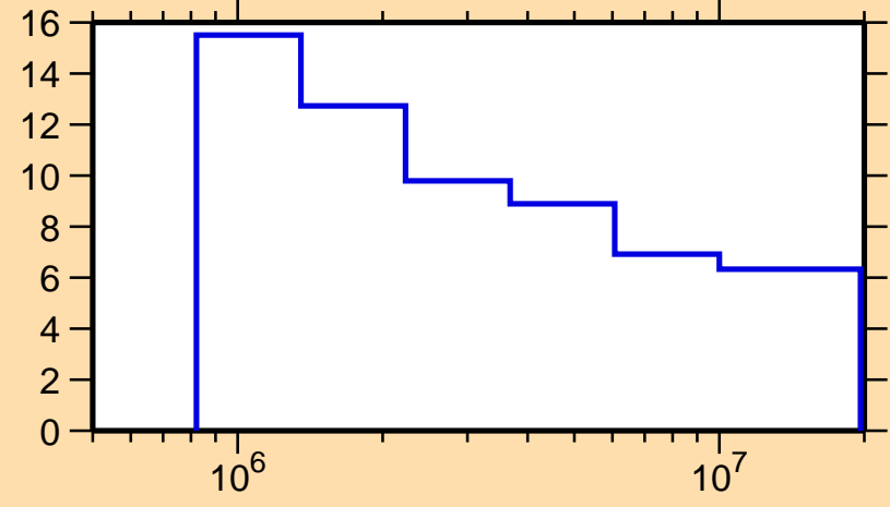
\Delta\sigma/\sigma vs. E for ^{103}\text{Ru}(n,n\text{onel.})
