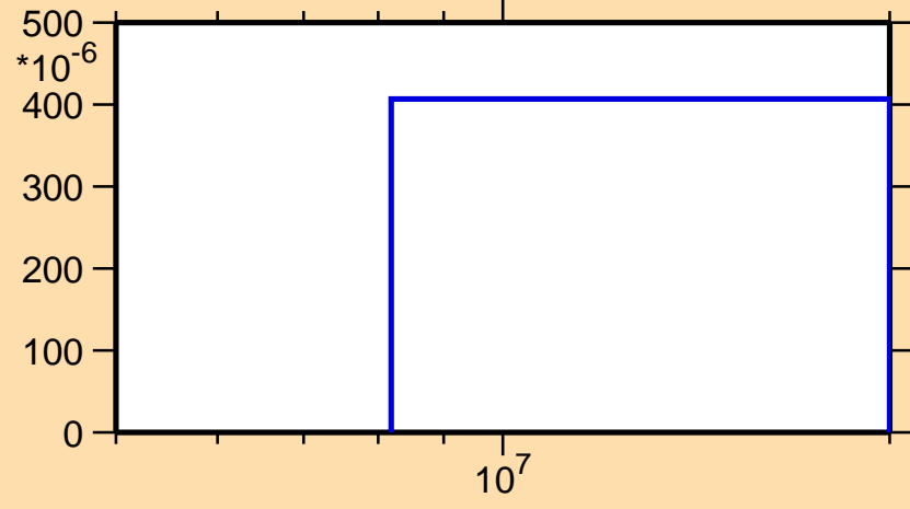
\sigma vs. E for ^{103}\text{Ru}(n,np)
