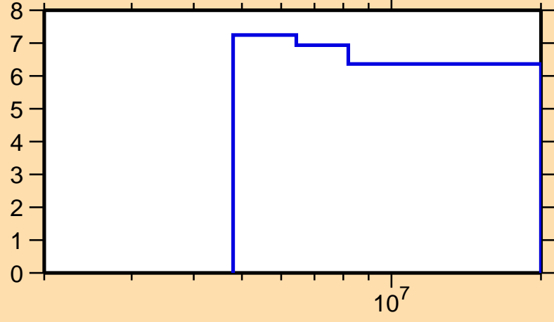
\Delta\sigma/\sigma vs. E for ^{103}\text{Ru}(n,\text{nonel.})
