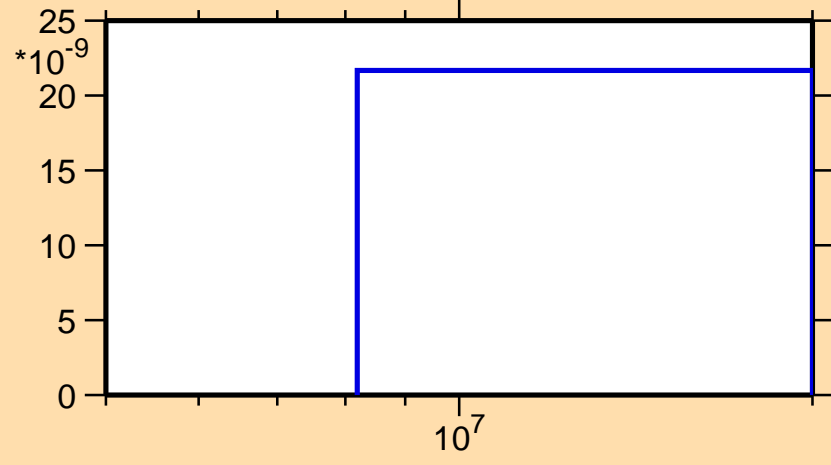
\sigma vs. E for ^{103}\text{Ru}(n,\text{nd})
