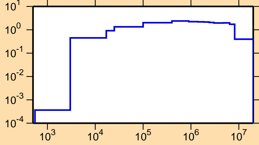
\sigma vs. E for ^{103}\text{Ru}(n,\text{inel.})
