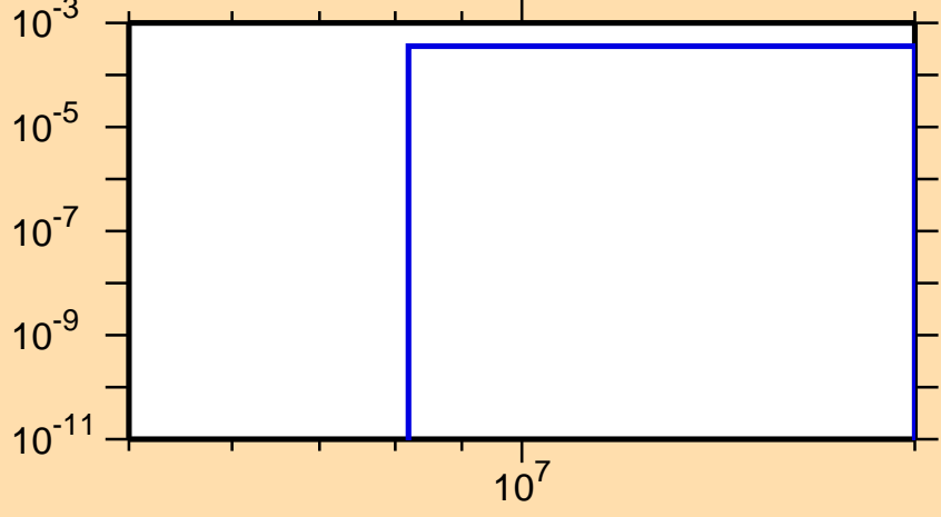
\sigma vs. E for ^{103}\text{Ru}(n,d)
