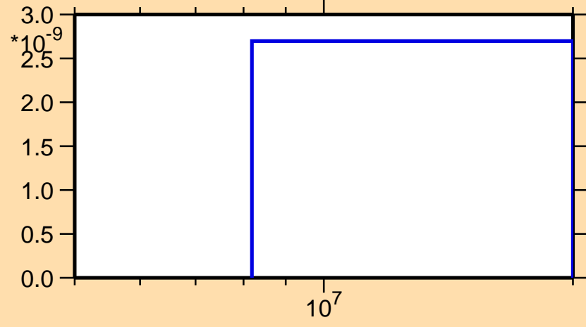
\sigma vs. E for ^{103}\text{Ru}(n,2n\alpha)
