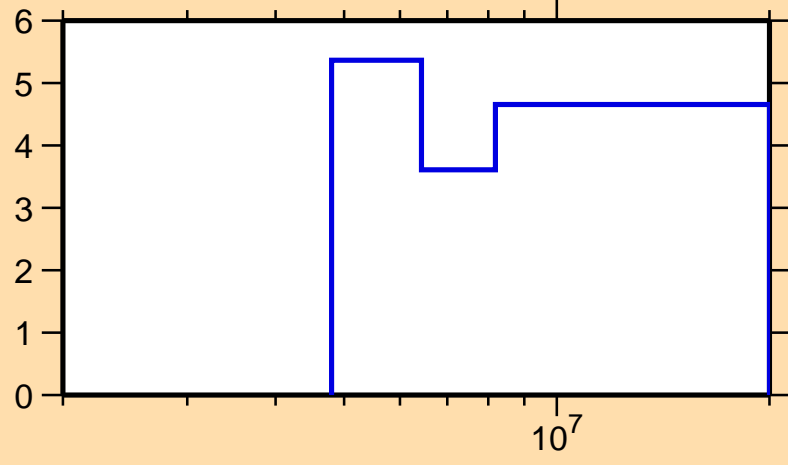
\Delta\sigma/\sigma vs. E for ^{103}\text{Ru}(n,\text{tot.})
