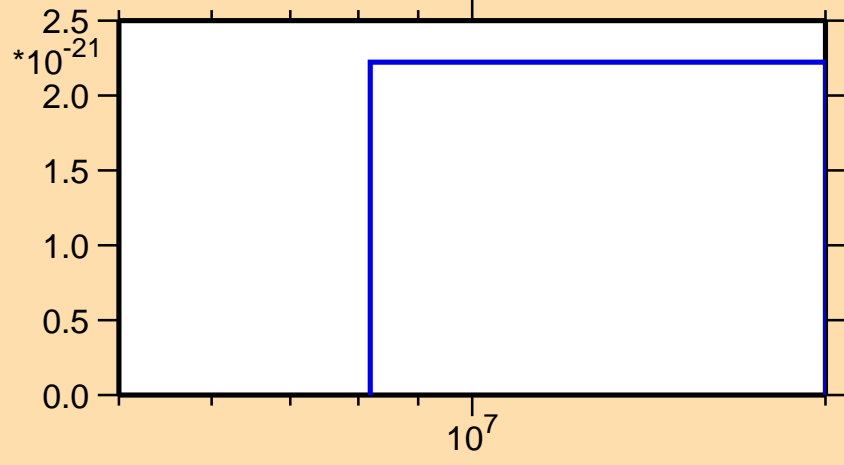
\sigma vs. E for ^{103}\text{Ru}(n,3n\alpha)
