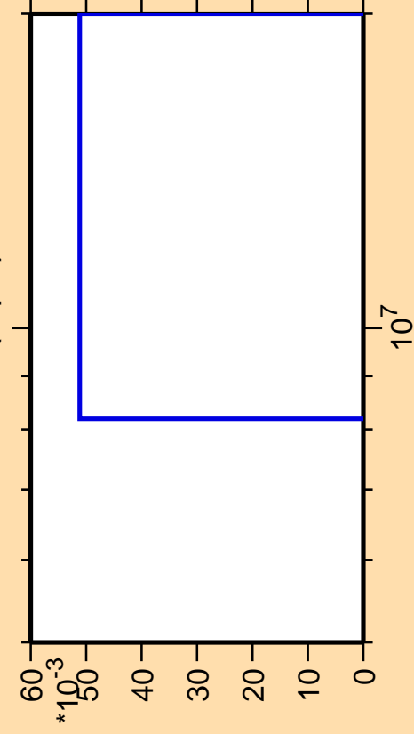
\Delta\sigma/\sigma vs. E for ^{103}\text{Ru}(n,p\alpha)
