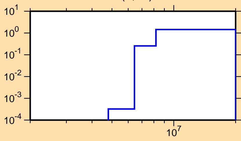
\sigma vs. E for ^{103}\text{Ru}(n,2n)
