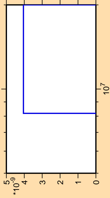
\Delta\sigma/\sigma vs. E for ^{103}\text{Ru}(n,3n\alpha)
