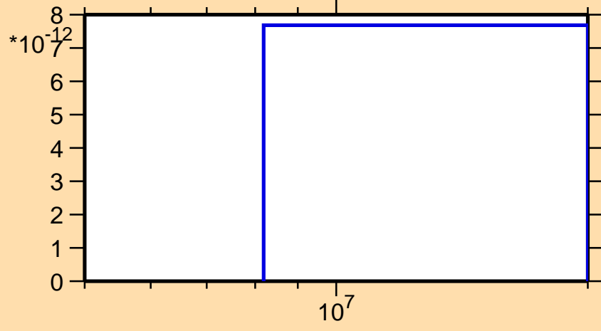
\sigma vs. E for ^{103}\text{Ru}(n,\text{He}3)
