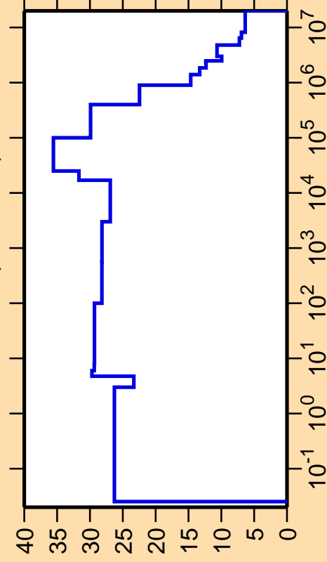
\Delta\sigma/\sigma vs. E for ^{103}\text{Ru}(n,\text{nonel.})
