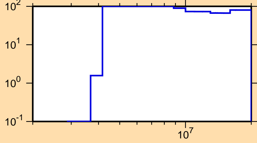
\Delta\sigma/\sigma vs. E for ^{105}\text{Ru}(n,p)
