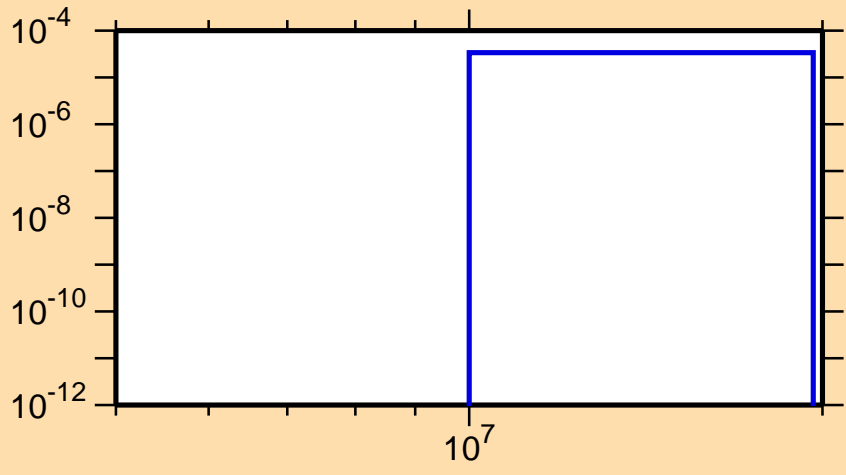
\sigma vs. E for ^{105}\text{Ru}(n,\alpha)
