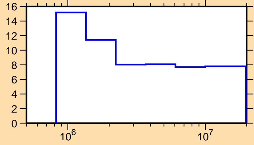
\Delta\sigma/\sigma vs. E for ^{105}\text{Ru}(n,n\text{onel.})
