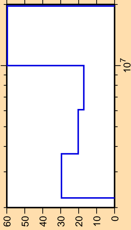
\Delta\sigma/\sigma vs. E for ^{106}\text{Ru}(n,\text{ncont.})
