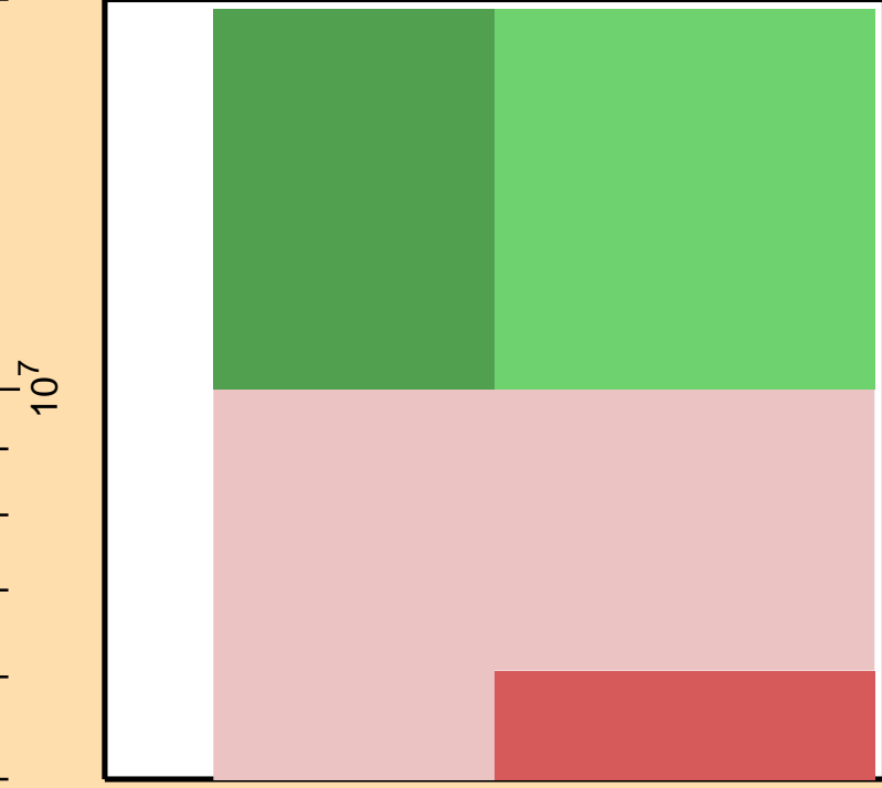
\Delta\sigma/\sigma vs. E for ^{106}\text{Ru}(n,2n)
