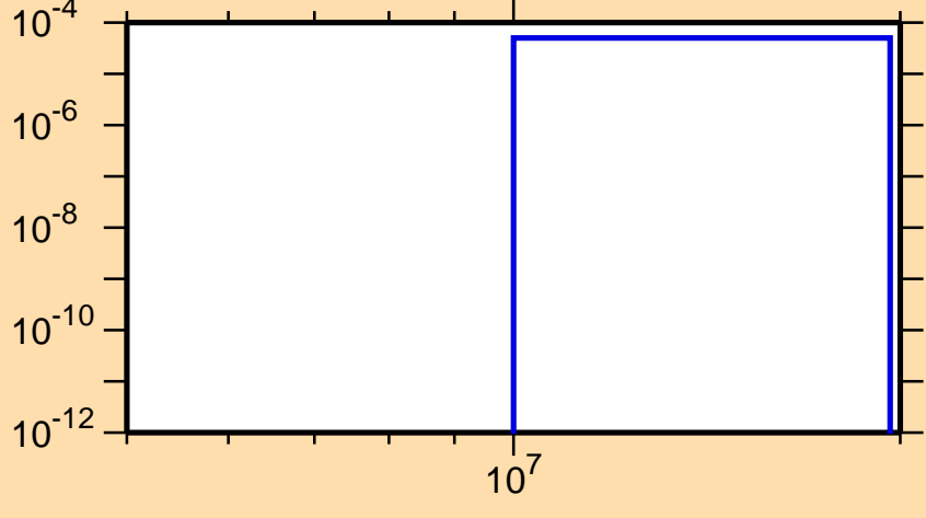
\sigma vs. E for ^{106}\text{Ru}(n,d)
