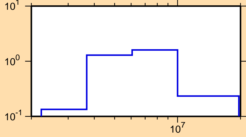
\sigma vs. E for ^{106}\text{Ru}(n,n\text{cont.})
