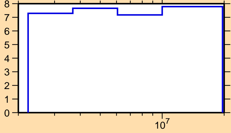
\Delta\sigma/\sigma vs. E for ^{106}\text{Ru}(n,n\text{onel.})
