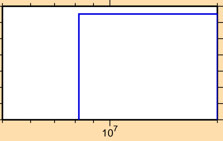
\sigma vs. E for ^{106}\text{Ru}(n,2n\alpha)
