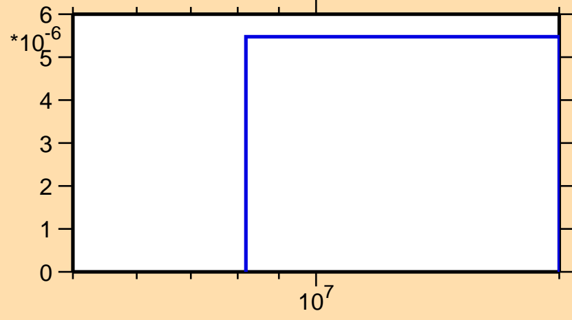
\sigma vs. E for ^{106}\text{Ru}(n,\alpha)
