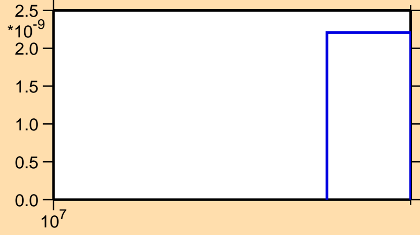
\sigma vs. E for ^{107}\text{Ru}(n,2np)
