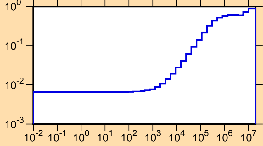
\mu vs. E for ^{107}\text{Ru}(\text{mt251})
