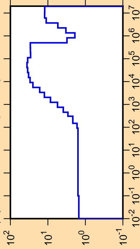
\Delta\mu/\mu vs. E for ^{107}\text{Ru}(\text{mt251})
