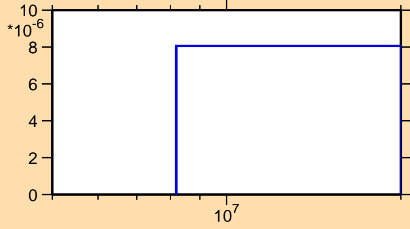
\sigma vs. E for ^{107}\text{Ru}(n,\alpha)
