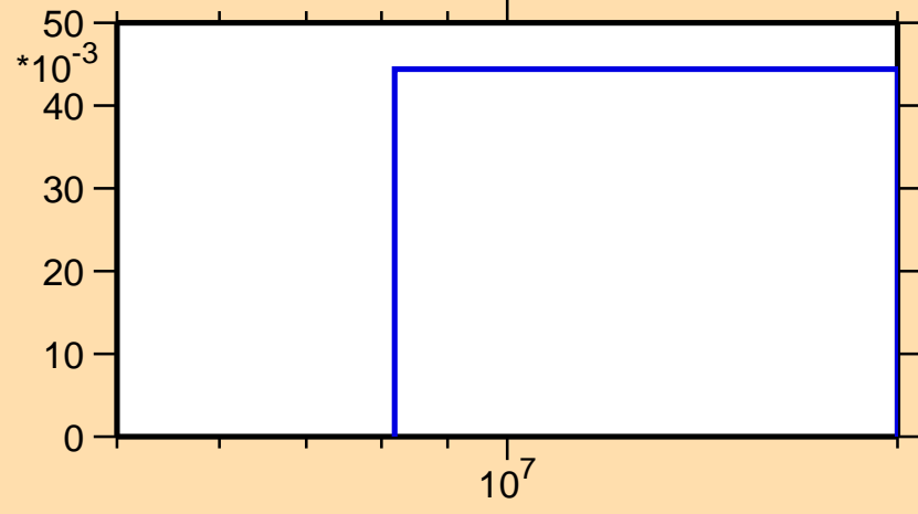
\sigma vs. E for ^{107}\text{Ru}(n,3n)
