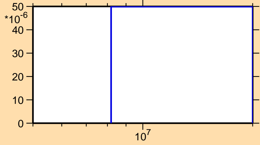
\sigma vs. E for ^{107}\text{Ru}(n,d)
