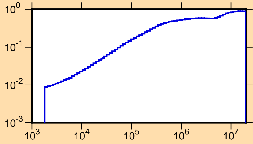
\mu vs. E for ^{108}\text{Ru}(\text{mt251})
