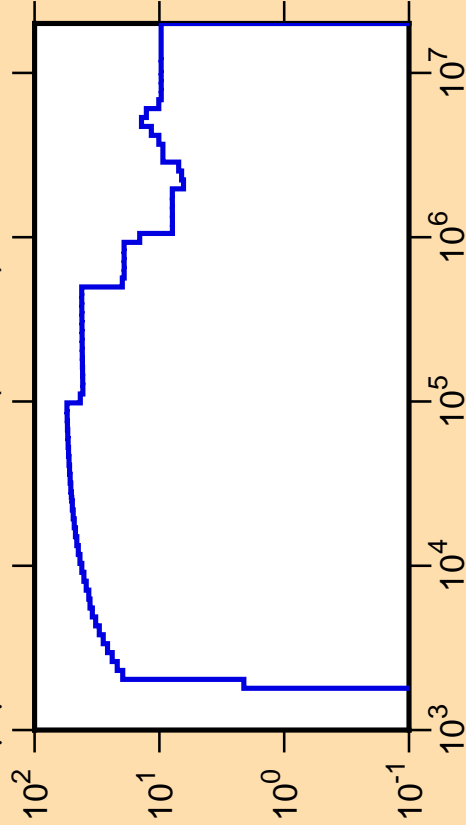
\Delta\mu/\mu vs. E for ^{108}\text{Ru}(\text{mt251})
