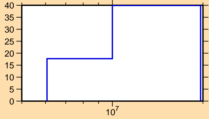
\Delta\sigma/\sigma vs. E for ^{108}\text{Ru}(n,ncont.)
