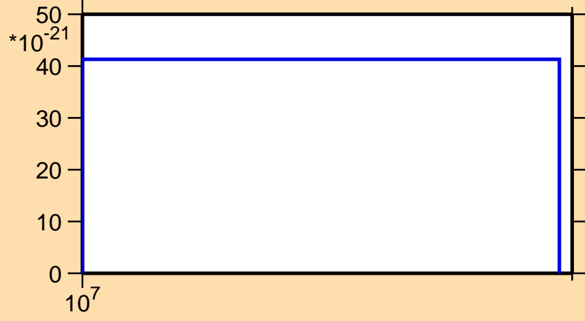
\sigma vs. E for ^{108}\text{Ru}(n,2np)
