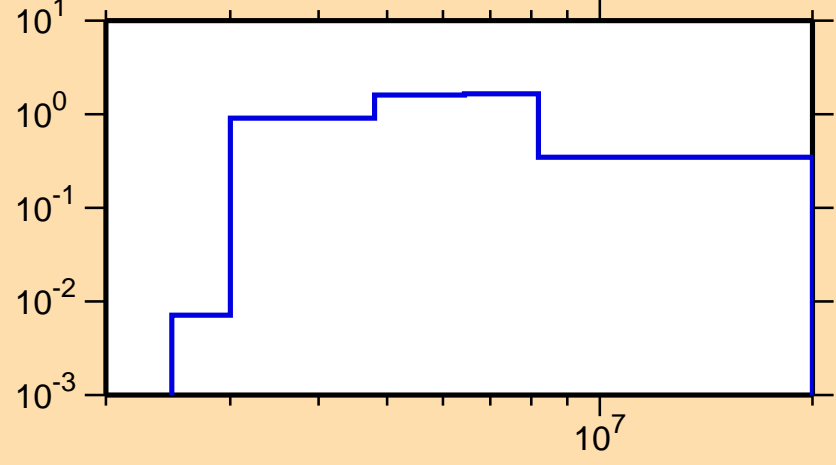
\sigma vs. E for ^{108}\text{Ru}(n,n\text{cont.})
