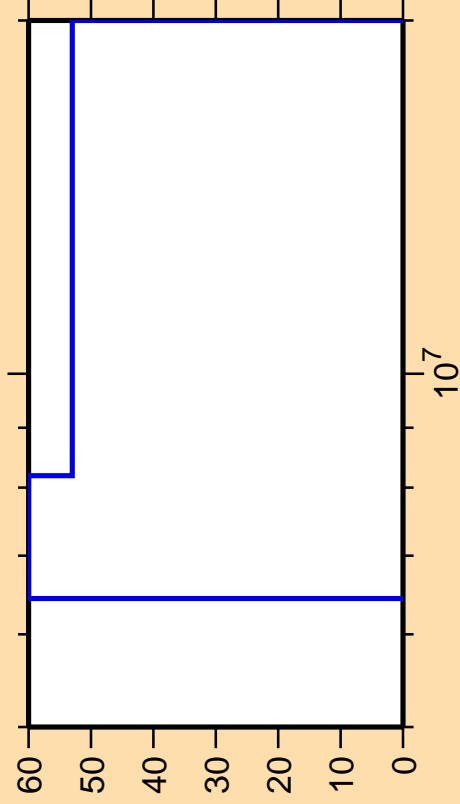
\Delta\sigma/\sigma vs. E for ^{108}\text{Ru}(n,\gamma)
