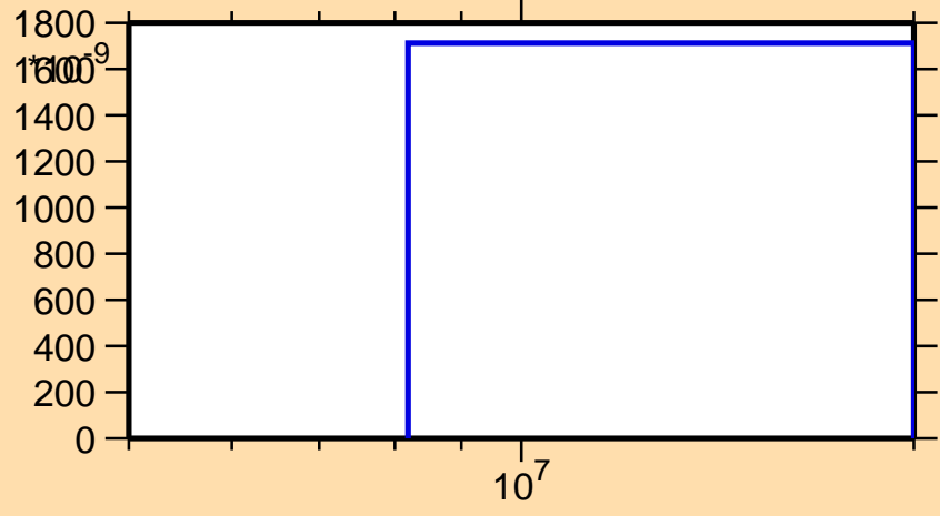
\sigma vs. E for ^{108}\text{Ru}(n,\alpha)
