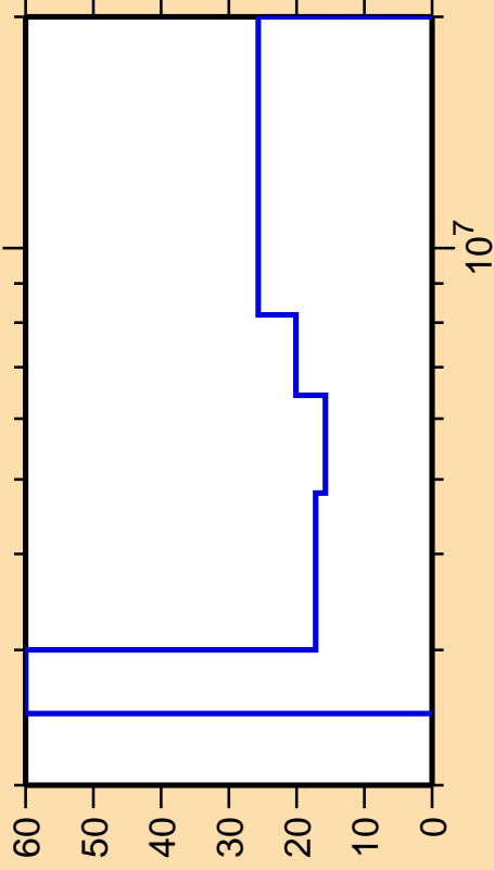
\Delta\sigma/\sigma vs. E for ^{108}\text{Ru}(n,\text{ncont.})
