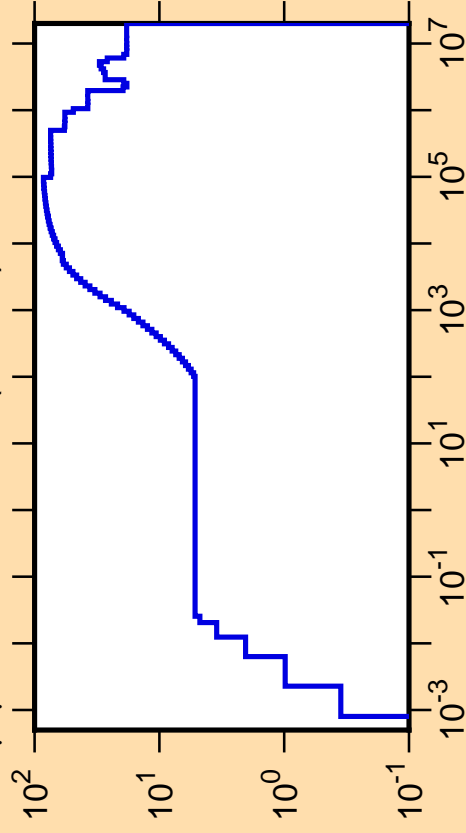
\Delta\mu/\mu vs. E for ^{109}\text{Ru}(\text{mt251})
