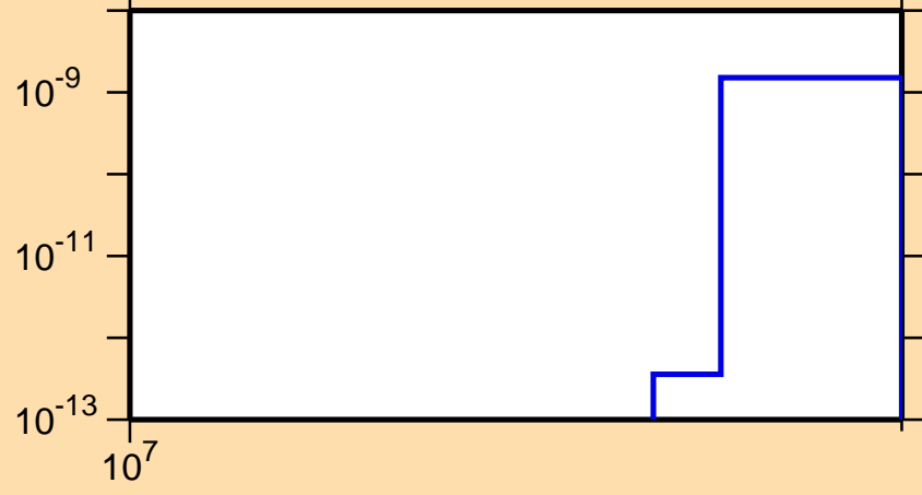
\sigma vs. E for ^{109}\text{Ru}(n,nt)
