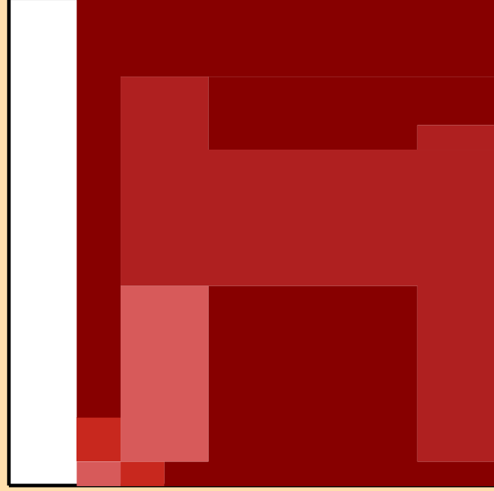
\Delta\sigma/\sigma vs. E for ^{109}\text{Ru}(n,p)
