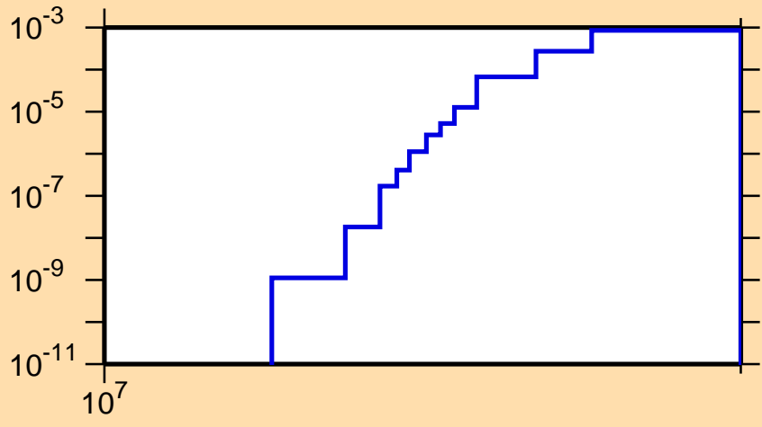
\sigma vs. E for ^{109}\text{Ru}(n,d)
