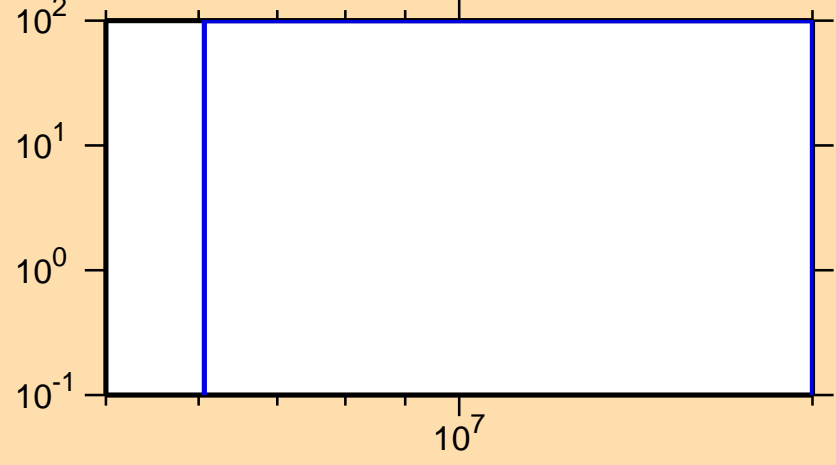
\Delta\sigma/\sigma vs. E for ^{109}\text{Ru}(n,n_1)
