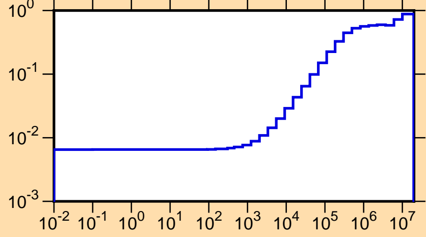
\mu vs. E for ^{109}\text{Ru}(\text{mt251})
