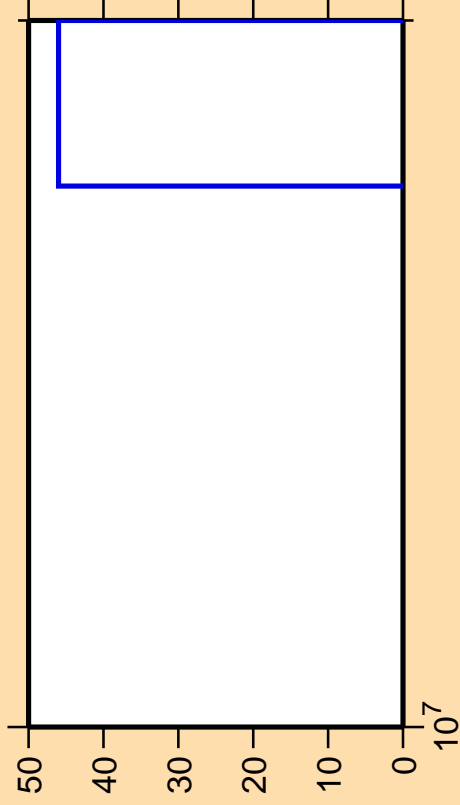
\Delta\sigma/\sigma vs. E for ^{110}\text{Ru}(n,\text{nd})
