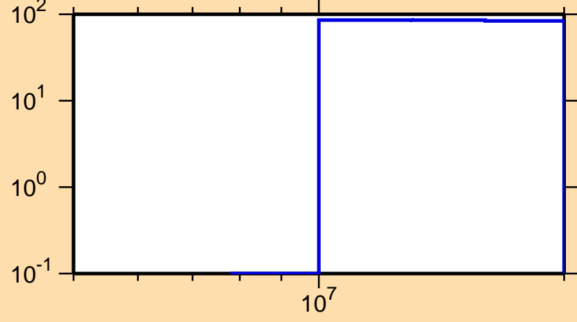
\Delta\sigma/\sigma vs. E for ^{110}\text{Ru}(n,p)
