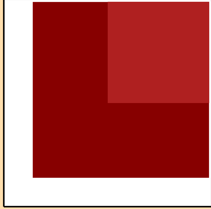
\Delta\sigma/\sigma vs. E for ^{110}\text{Ru}(n,p)
