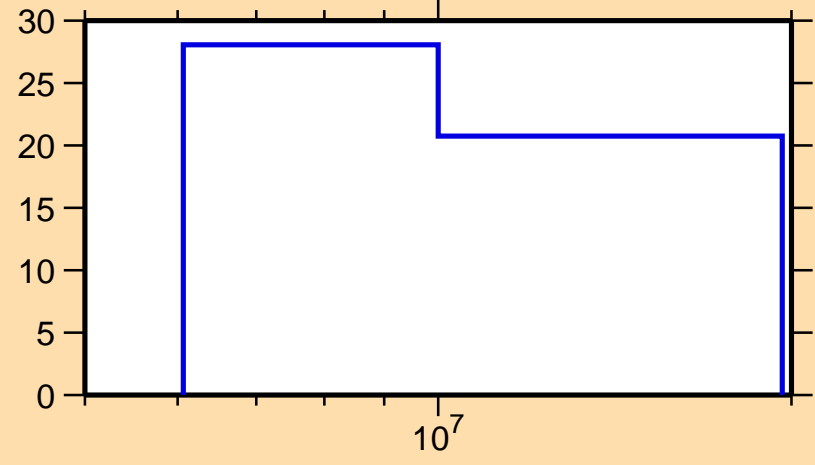
\Delta\sigma/\sigma vs. E for ^{110}\text{Ru}(n,el.)
