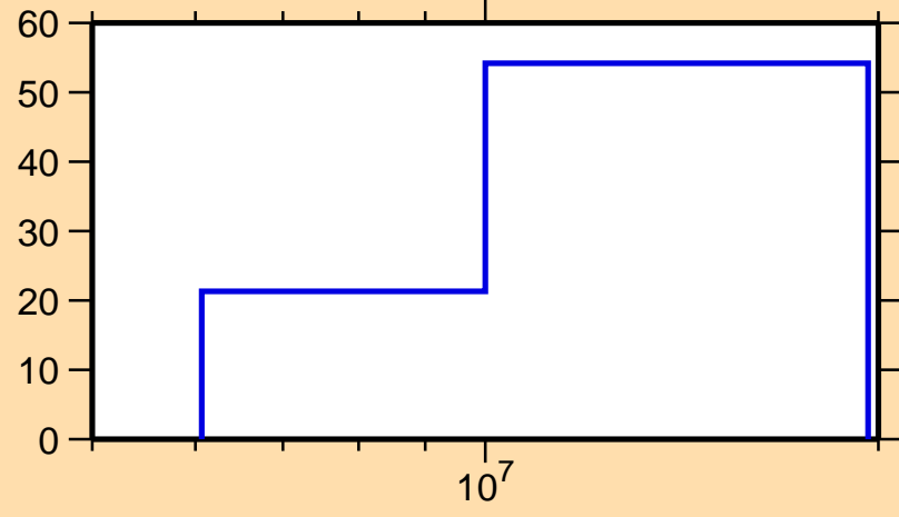
\Delta\sigma/\sigma vs. E for ^{110}\text{Ru}(n,n\text{cont.})
