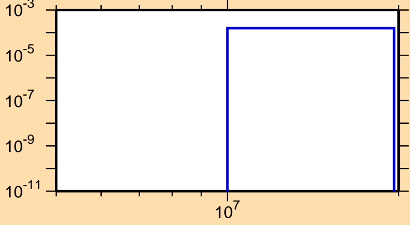
\sigma vs. E for ^{110}\text{Ru}(n,p)
