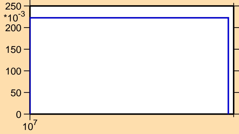
\sigma vs. E for ^{110}\text{Ru}(n,3n)
