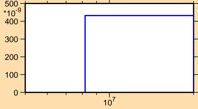
\sigma vs. E for ^{110}\text{Ru}(n,t)
