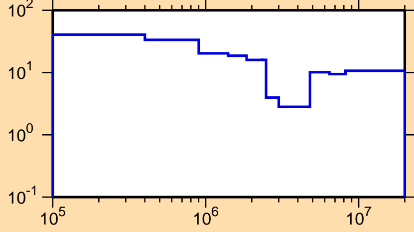
\Delta\sigma/\sigma vs. E for ^{110}\text{Ru}(n,\text{nonel.})
