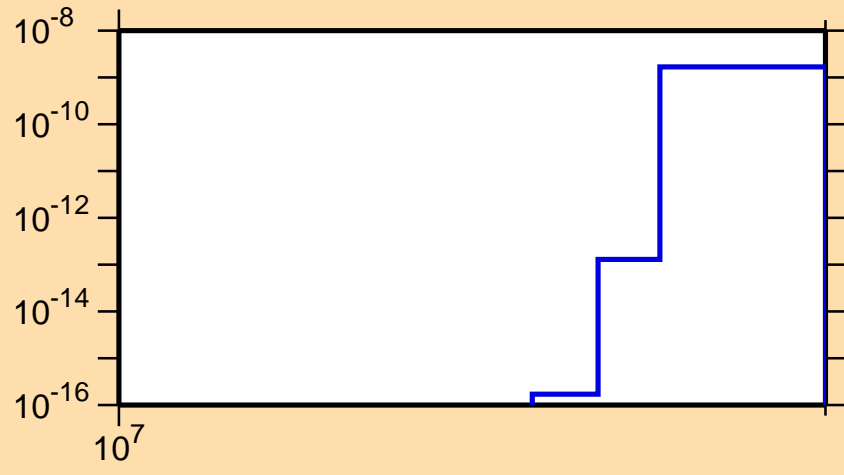
\sigma vs. E for ^{111}\text{Ru}(n,nt)
