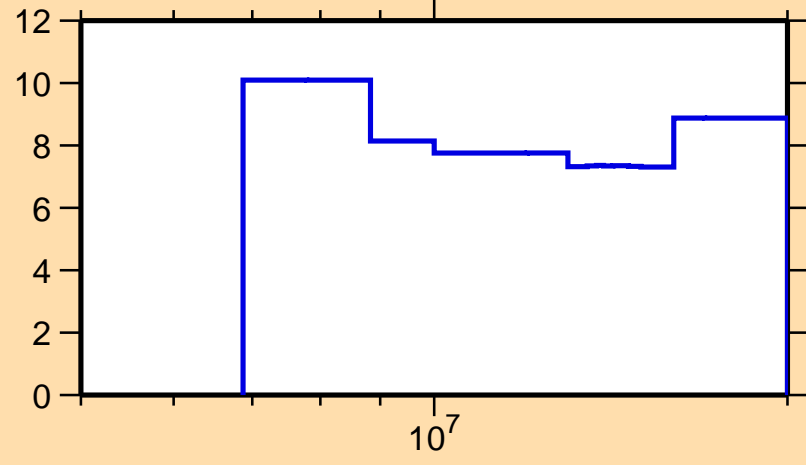
\Delta\sigma/\sigma vs. E for ^{111}\text{Ru}(n,\text{nonel.})
