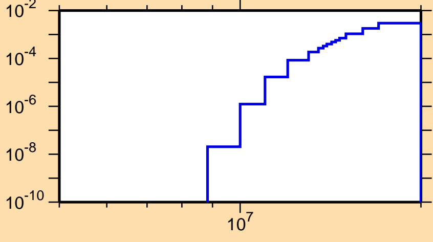
\sigma vs. E for ^{111}\text{Ru}(n,p)
