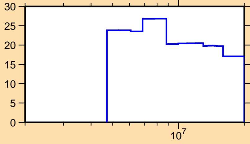
\Delta\sigma/\sigma vs. E for ^{111}\text{Ru}(n,\text{inel.})
