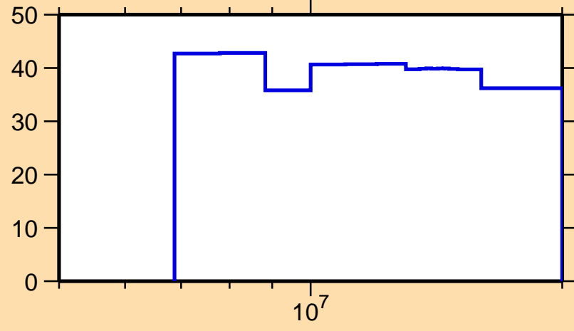
\Delta\sigma/\sigma vs. E for ^{111}\text{Ru}(n,ncont.)
