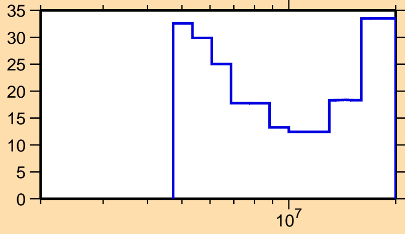
\Delta\sigma/\sigma vs. E for ^{111}\text{Ru}(n,2n)
