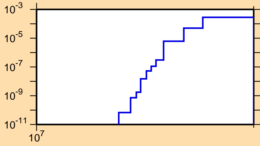
\sigma vs. E for ^{111}\text{Ru}(n,d)
