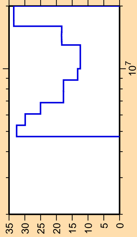
\Delta\sigma/\sigma vs. E for ^{111}\text{Ru}(n,2n)
