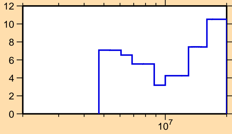
\Delta\sigma/\sigma vs. E for ^{111}\text{Ru}(n,\text{tot.})
