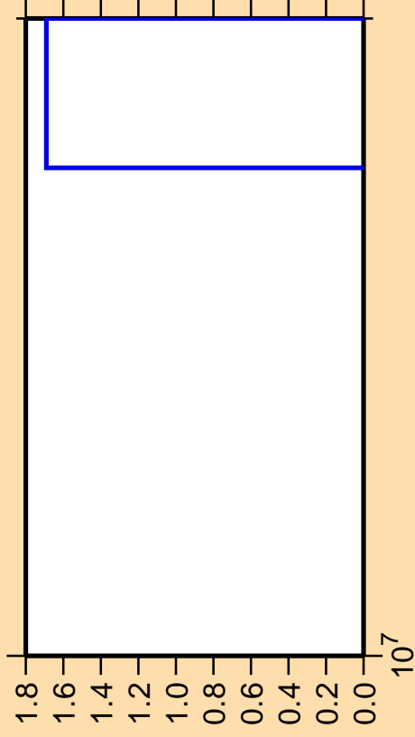
\Delta\sigma/\sigma vs. E for ^{111}\text{Ru}(n,2np)
