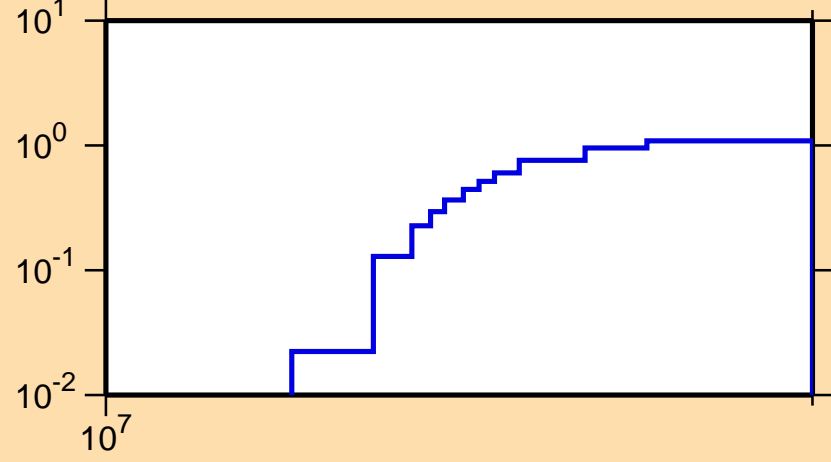
\sigma vs. E for ^{111}\text{Ru}(n,3n)
