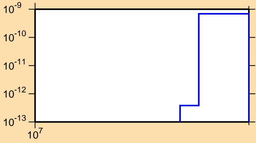
\sigma vs. E for ^{111}\text{Ru}(n,2n\alpha)
