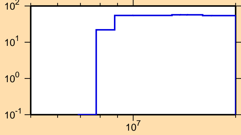
\Delta\sigma/\sigma vs. E for ^{111}\text{Ru}(n,p)
