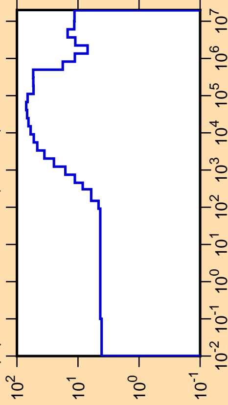
\Delta\mu/\mu vs. E for ^{111}\text{Ru}(\text{mt251})
