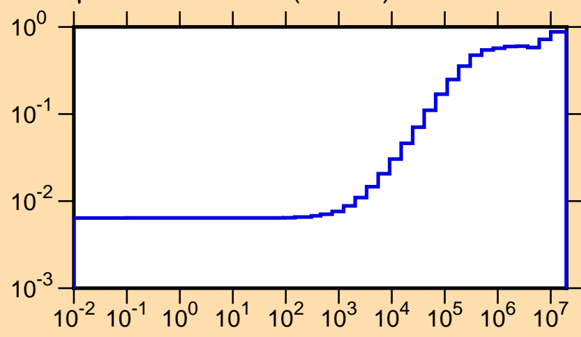
\mu vs. E for ^{111}\text{Ru}(\text{mt251})
