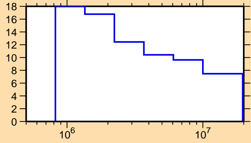
\Delta\sigma/\sigma vs. E for ^{111}\text{Ru}(n,n\text{onel.})
