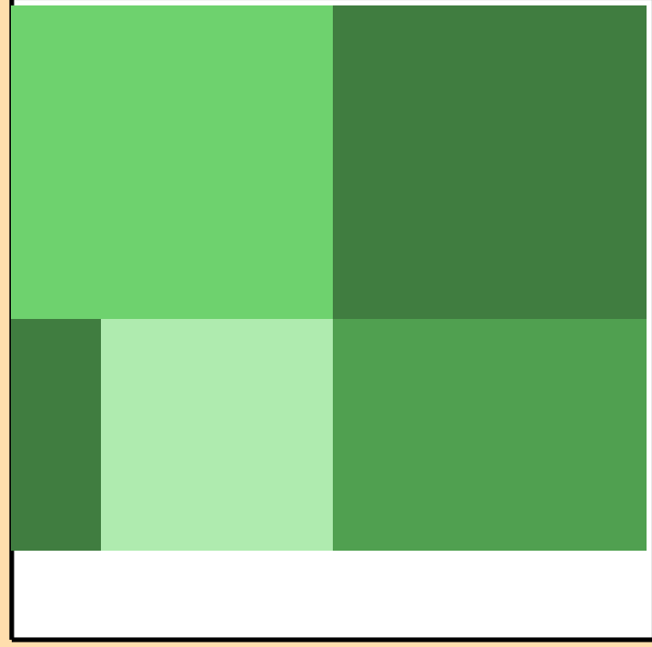
\Delta\sigma/\sigma vs. E for ^{111}\text{Ru}(n,\gamma)
