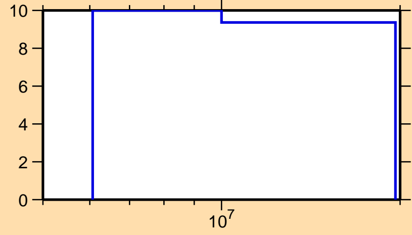
\Delta\sigma/\sigma vs. E for ^{111}\text{Ru}(n,el.)
