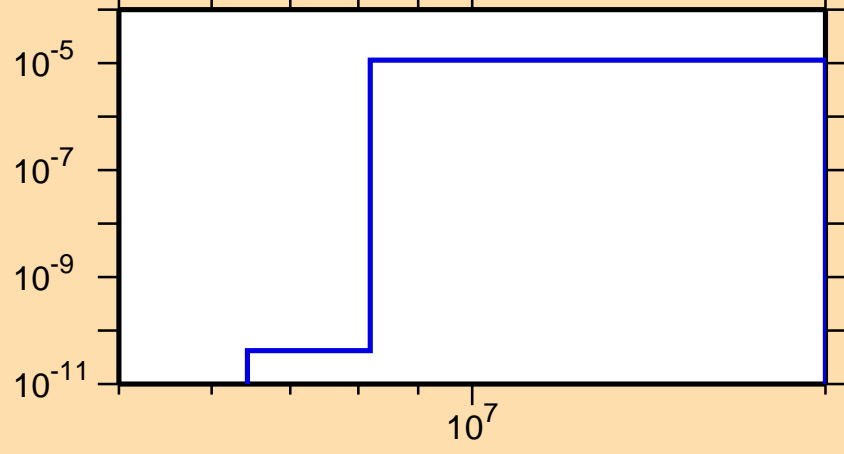
\sigma vs. E for ^{111}\text{Ru}(n,\alpha)
