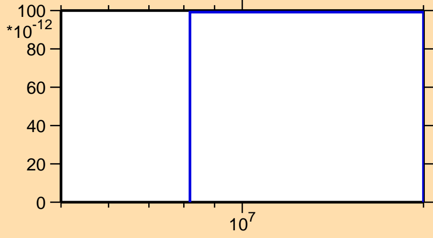
\sigma vs. E for ^{111}\text{Ru}(n,\text{nd})
